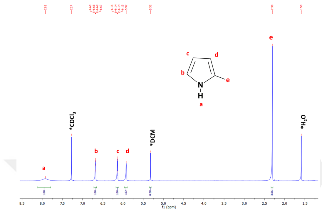
Figure 4.2 ^1\text{H} NMR spectrum of 2-methylpyrrole in \text{CDCl}_3 at room temperature. \text{CDCl}_3 , \text{H}_2\text{O} , and dichloromethane (DCM) peaks originating from the NMR-solvent are denoted by asterisks.
