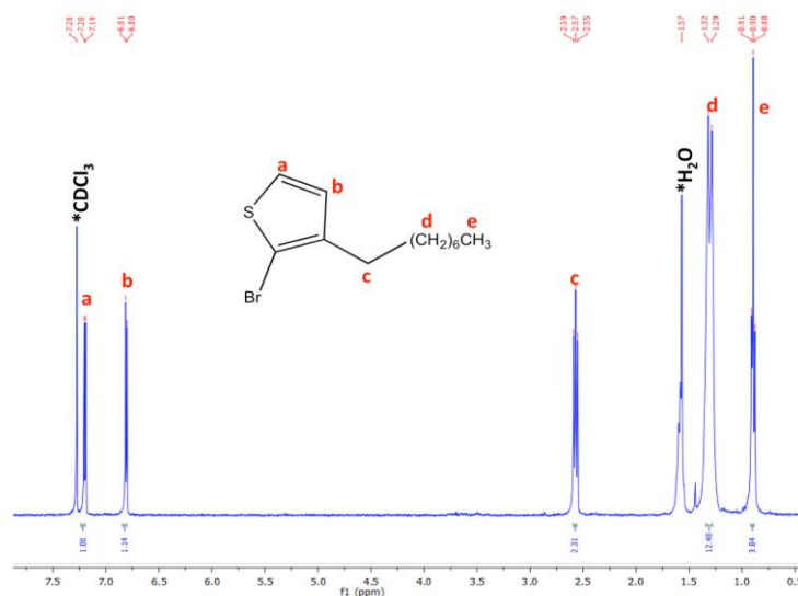
Figure 3.7 ^1\text{H} NMR spectra of 4 in \text{CDCl}_3 at room temperature. (Bruker 400/Erciyes University-TAUM). ( \text{CDCl}_3 peak and \text{H}_2\text{O} peak in NMR solvent are denoted by asterisks).
