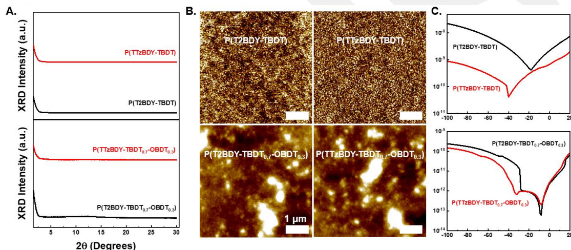
Figure 4.40 (A) \theta -2 \theta X-ray diffraction (XRD) profiles and (B) AFM topographic images for thin films of P(T2BDY-TBDT) , P(TTzBDY-TBDT) , P(T2BDY-TBDT 0.7 -OBDT 0.3 ) , and P(TTzBDY-TBDT 0.7 -OBDT 0.3 ) . (C) Transfer curves showing p -type characteristics ( V_{DS} = -100 V) for (BG/TC) OFET devices fabricated with spin-coated copolymer thin films.
