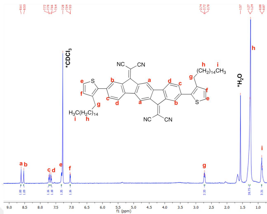
Figure 3.24 1 H NMR spectra of \beta,\beta' -C16-TIFDMT in \text{CDCl}_3 at room temperature. (Bruker 400/Erciyes University-TAUM). ( \text{CDCl}_3 peak and \text{H}_2\text{O} peak in NMR solvent are denoted by asterisks).
