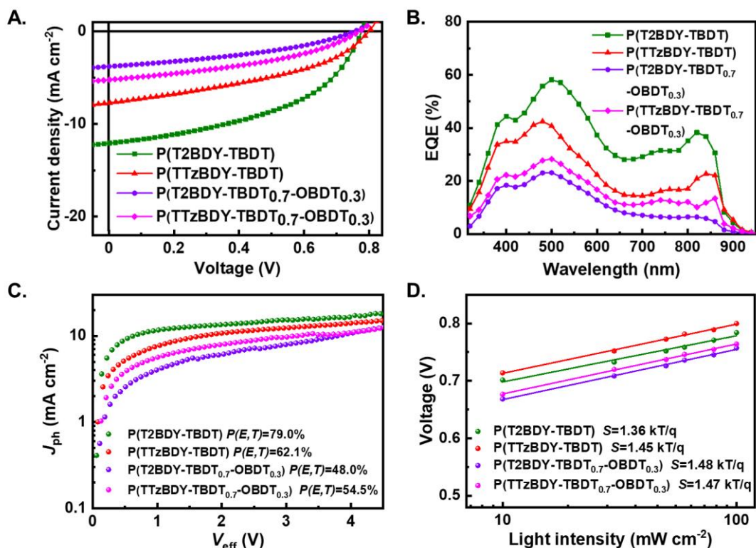
Figure 4.41 (A) Current density–voltage ( J – V ) curves, (B) external quantum efficiency (EQE) curves, (C) exciton dissociation probabilities ( P(E, T) s), and (D) P_{light} -dependent V_{oc} characteristics for BHJ solar cells fabricated with P(T2BDY-TBDT) , P(TTzBDY-TBDT) , P(T2BDY-TBDT 0.7 -OBDT 0.3 ) , and P(TTzBDY-TBDT 0.7 -OBDT 0.3 ) donor polymers.
