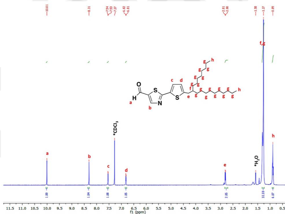
Figure 4.15 1 H NMR spectrum of 20D-TTz-COH in CDCl 3 at room temperature. CDCl 3 and H 2 O peaks originating from the NMR-solvent are denoted by asterisks.
