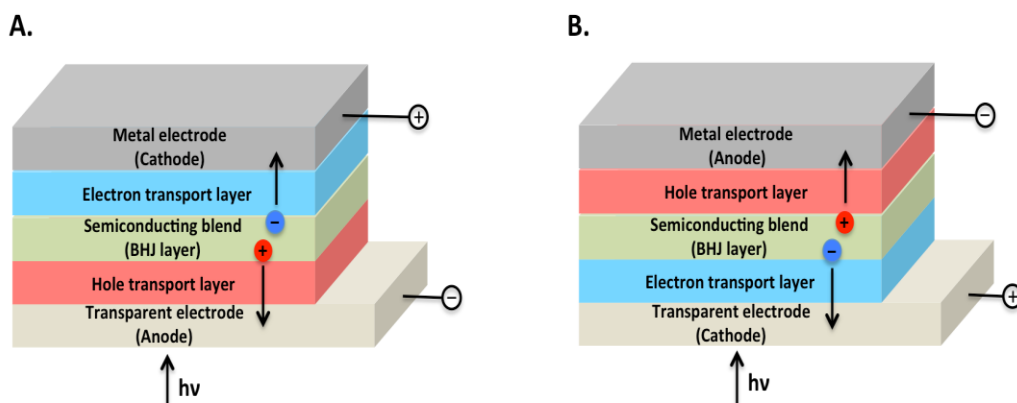
Figure 1.3 The pictorial representation of regular OPV device architecture (A) and inverted OPV device architecture (B).
