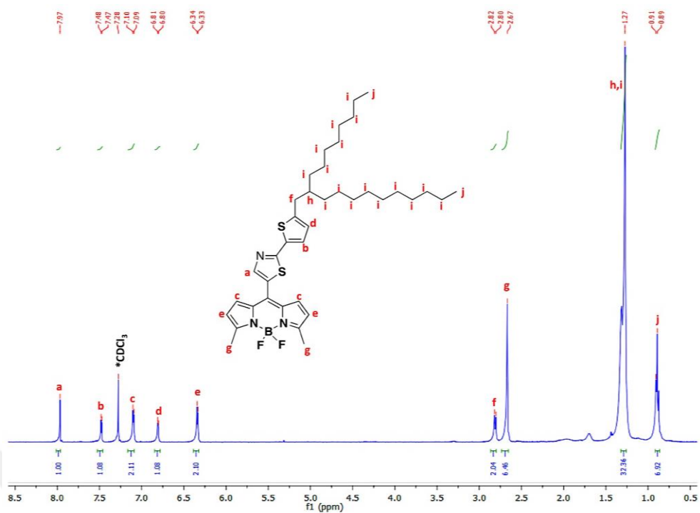
Figure 4.16 ^1\text{H} NMR spectrum of 2OD-TTzBDY in \text{CDCl}_3 at room temperature. \text{CDCl}_3 peak originating from the NMR-solvent is denoted by asterisk.
