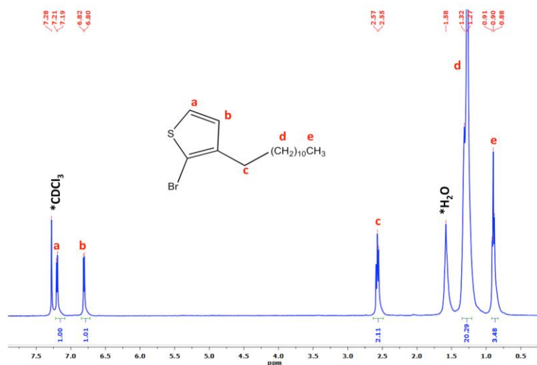
Figure 3.14 ^1\text{H} NMR spectra of 8 in \text{CDCl}_3 at room temperature. (Bruker 400/Erciyes University-TAUM). ( \text{CDCl}_3 peak and \text{H}_2\text{O} peak in NMR solvent are denoted by asterisks).
