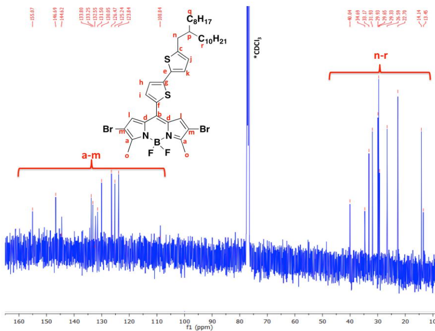
Figure 4.9 13 C NMR spectrum of 2OD-T2BDY-Br 2 in CDCl 3 at room temperature. CDCl 3 peak originating from the NMR-solvent is denoted by asterisks.
