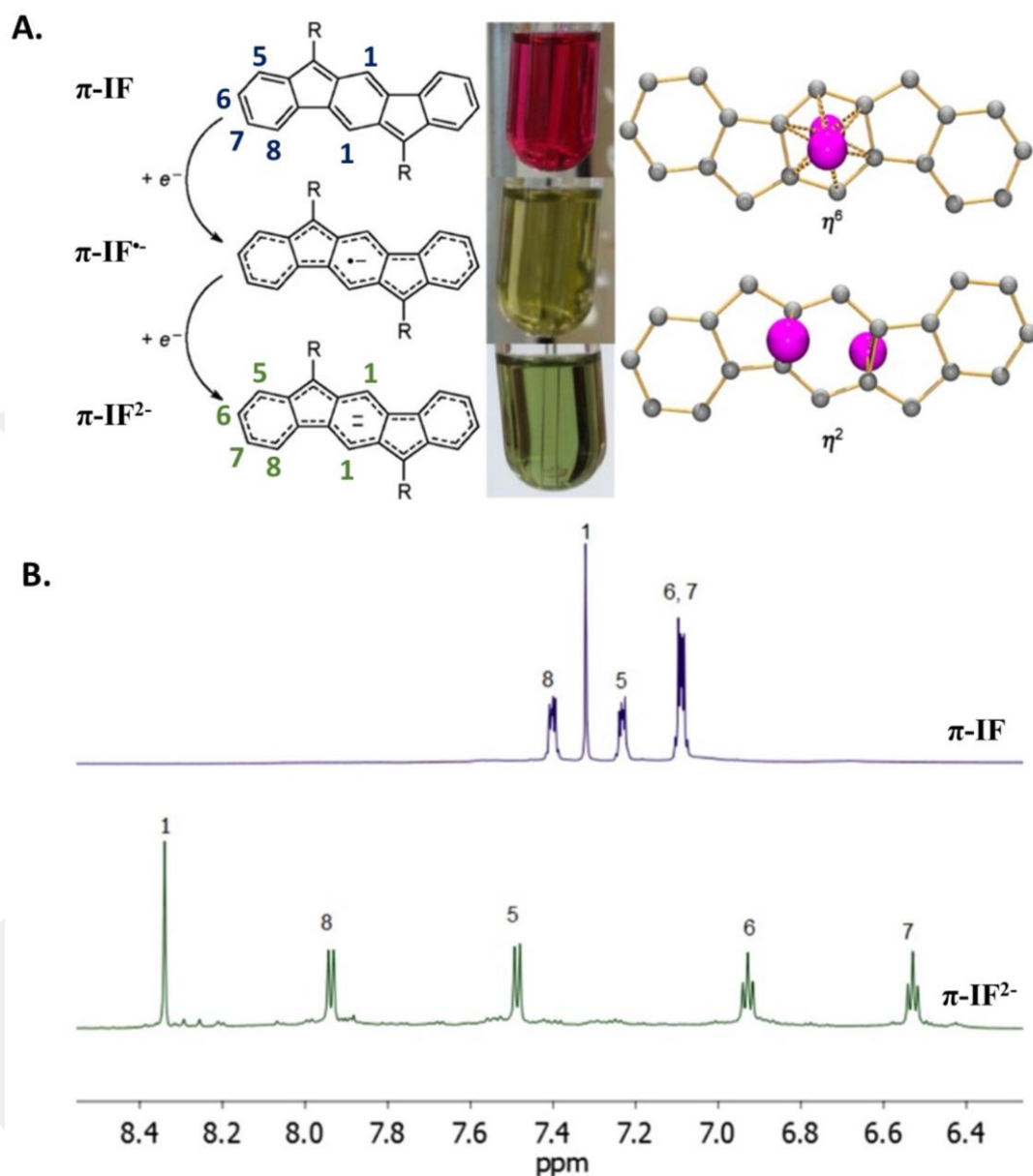
Figure 2.20 A. One- and two-electron reduction processes for a representative \pi -IF core, the corresponding solution colors for neutral ( \pi -IF), anion radical ( \pi -IF ^{\bullet-} ), and dianion ( \pi -IF ^{2-} ) forms, and close-up views of \pi -IF ^{2-} s in the single-crystal structure with Rb^+ ions (in pink) that are \eta^2 - and \eta^6 -coordinated to the central six-membered ring (hydrogens are omitted for clarity). B. Partial ^1H NMR spectra of neutral \pi -IF-4a and dianion \pi -IF-4a ^{2-} in THF- d_8 with assigned hydrogen positions [112]. Reprinted with permission from reference 112. Copyright 2014, American Chemical Society.
