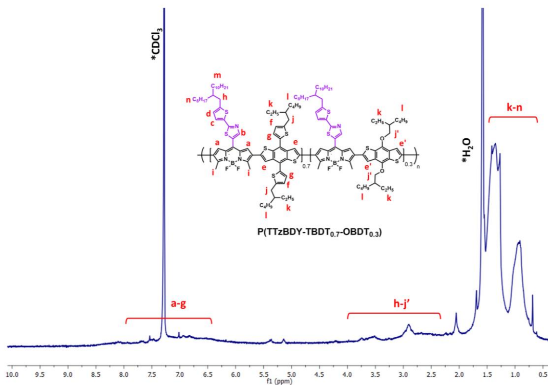
Figure 4.28 ^1H NMR spectrum of P(TTzBDY-TBDT_{0.7}-OBDT_{0.3}) in CDCl_3 at room temperature. CDCl_3 and H_2O peaks originating from the NMR-solvent are denoted by asterisks.
