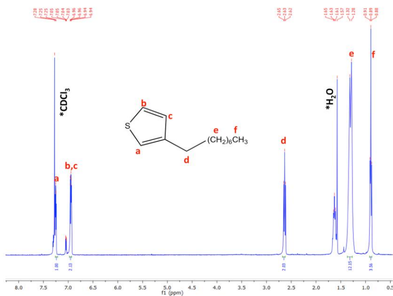
Figure 3.6 ^1\text{H} NMR spectra of 3 in \text{CDCl}_3 at room temperature. (Bruker 400/Erciyes University-TAUM). ( \text{CDCl}_3 peak and \text{H}_2\text{O} peak in NMR solvent are denoted by asterisks).
