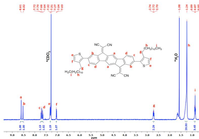
Figure 3.17 ^1\text{H} NMR spectra of \beta,\beta' -C12-TIFDMT in \text{CDCl}_3 at room temperature. (Bruker 400/Erciyes University-TAUM). ( \text{CDCl}_3 peak and \text{H}_2\text{O} peak in NMR solvent are denoted by asterisks).
