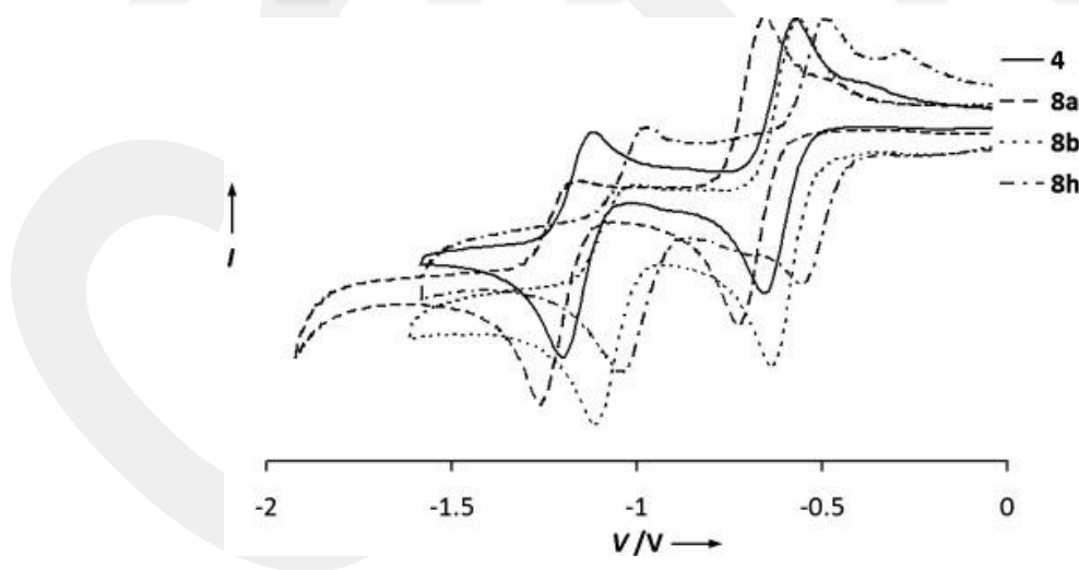
Figure 2.23 Cyclic voltammograms of \pi -IF-3a (4 in the figure), \pi -IF-4a (8a in the figure), \pi -IF-4b (8b in the figure), and \pi -IF-4h (8h in the figure) showing normalized reduction peaks [124]. Reprinted with permission from reference 124. Copyright 2011, Wiley-VCH.
