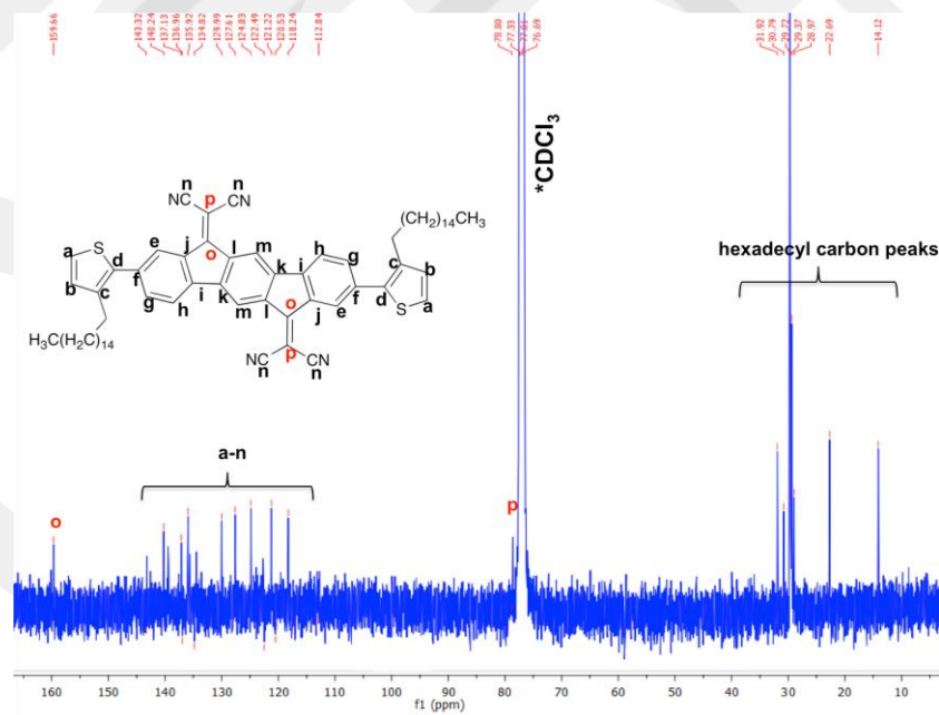
Figure 3.25 13 C NMR spectra of \beta,\beta' -C16-TIFDMT in \text{CDCl}_3 at room temperature. (Bruker 400/Erciyes University-TAUM). ( \text{CDCl}_3 peak in NMR solvent is denoted by asterisks).
