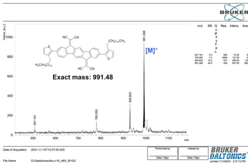
Figure 3.26 Positive ion and linear mode MALDI TOF-MS spectrum of C16-TIFDMT .
