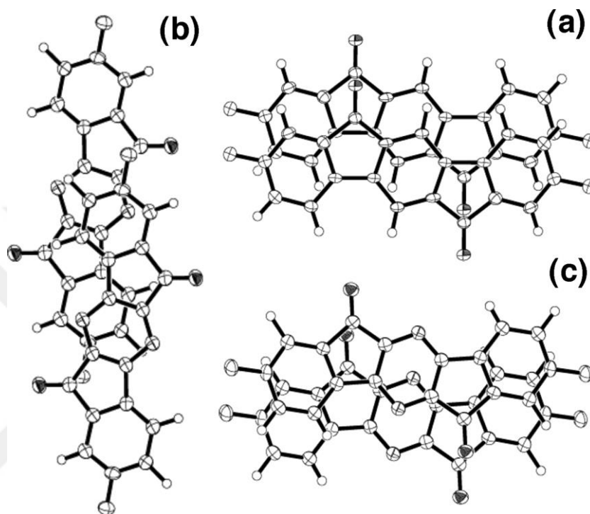
Figure 2.6 Dimeric packing motifs of IF-dione-5a (a) and IF-dione-6b (b: red-crystal and c: black-crystal) in single crystals [71]. Reprinted with permission from reference 71. Copyright 2008, American Chemical Society.
