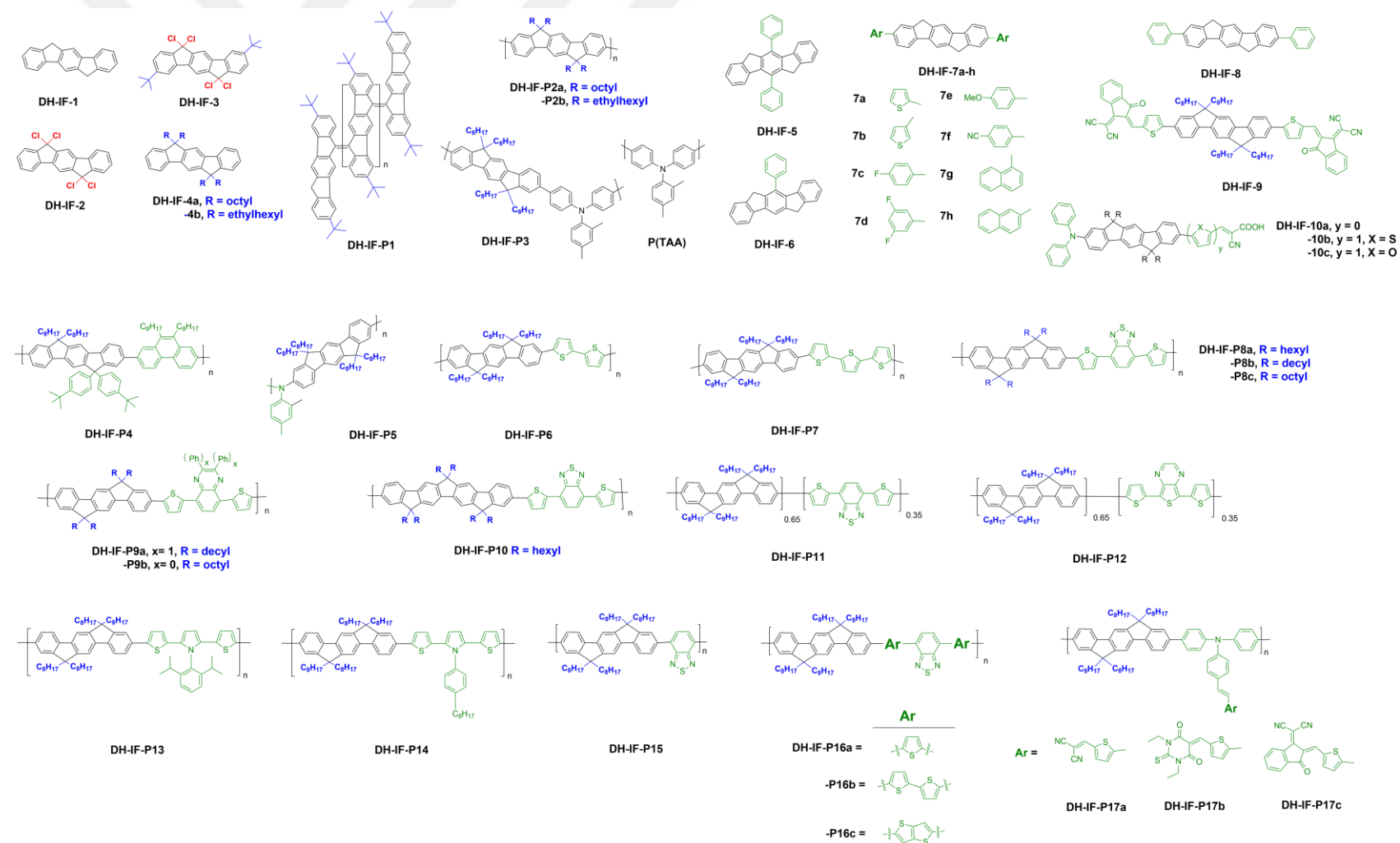
Figure 2.30 Chemical structures of (un)substituted dihydroindenofluorenes (DH-IFs)-based semiconductors DH-IFs-1-10 and DH-IFs-P1-P17 .
