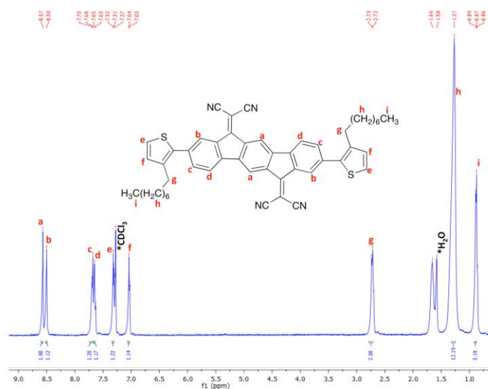
Figure 3.10 ^1\text{H} NMR spectra of \beta,\beta' -C8-TIFDMT in \text{CDCl}_3 at room temperature. (Bruker 400/Erciyes University-TAUM). ( \text{CDCl}_3 peak and \text{H}_2\text{O} peak in NMR solvent are denoted by asterisks).
