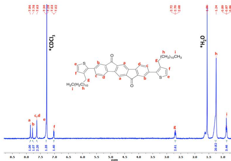
Figure 3.16 ^1\text{H} NMR spectra of 10 in \text{CDCl}_3 at room temperature. (Bruker 400/Erciyes University-TAUM). ( \text{CDCl}_3 peak and \text{H}_2\text{O} peak in NMR solvent are denoted by asterisks).
