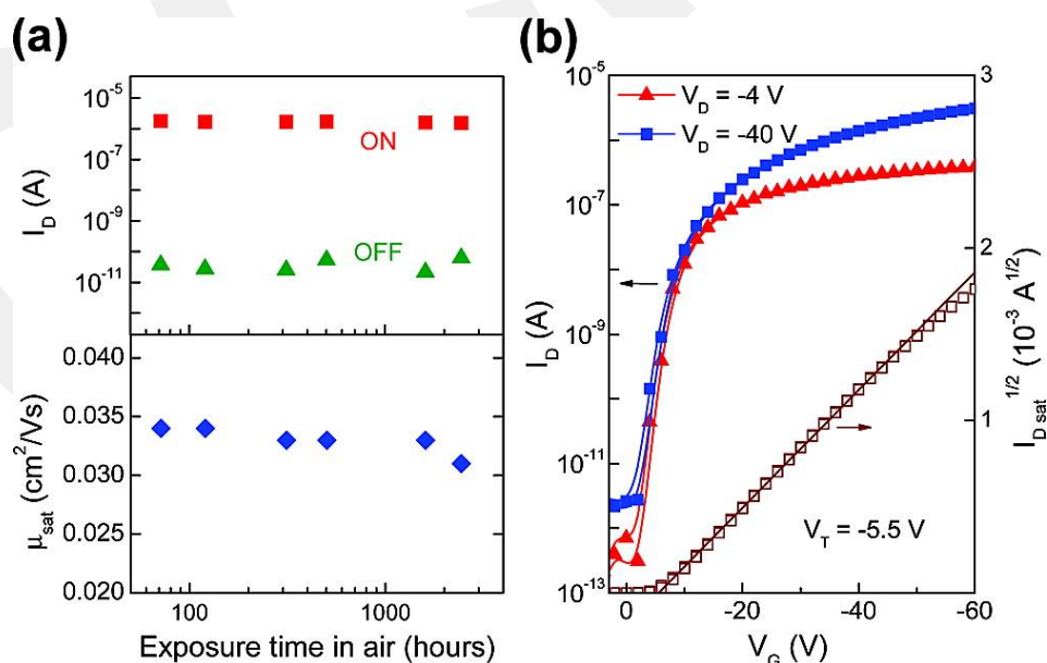
Figure 2.33 (a) I_{\text{on}} - I_{\text{off}} currents (top) and saturated hole mobilities (bottom) measured for DH-IF-P3 -based OFETs upon storage in air over a period of \sim 3 months. (b) Transfer characteristics for DH-IF-P3 -based OFETs ( W/L = 1000 \text{ }\mu\text{m}/30 \text{ }\mu\text{m} ) measured
