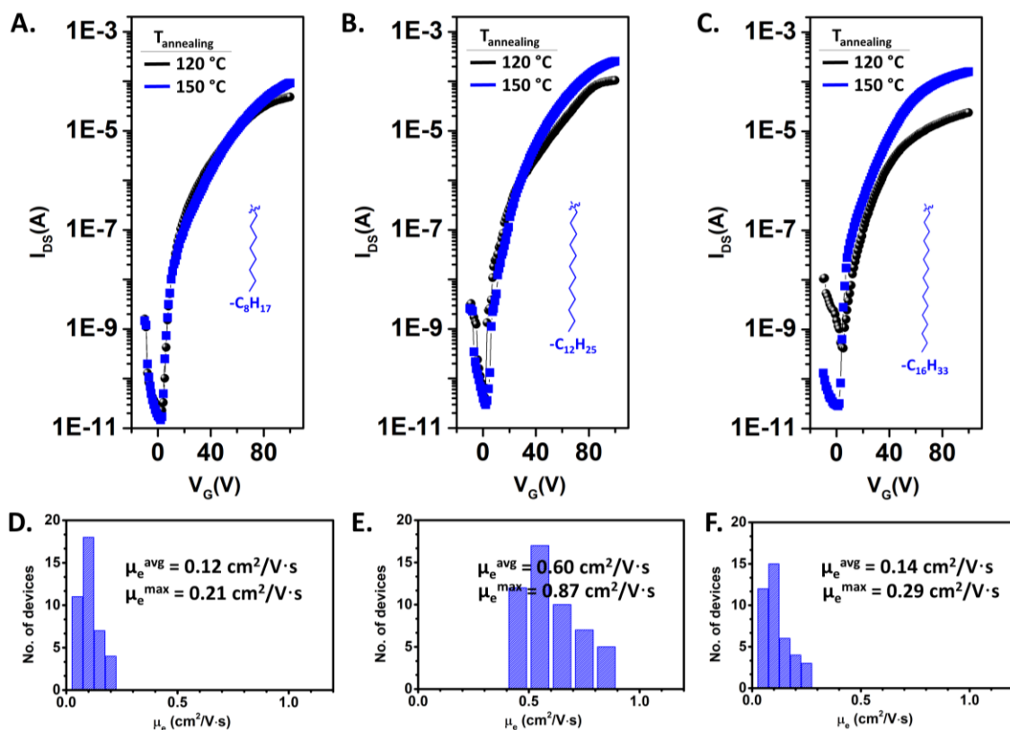
Figure 3.33 Transfer plots ( V_{DS} = 100 V) measured in ambient for p ++ -Si/SiO 2 /PS-brush( M_n = 5 kDa)/semiconductor/Au OFET devices fabricated based on the semiconductor molecules \beta,\beta' -C 8 -TIFDMT (A), \beta,\beta' -C 12 -TIFDMT (B), and \beta,\beta' -C 16 -TIFDMT (C), and the corresponding statistical distribution of \mu_e 's (D, E, and F, respectively) based on the number of measured devices (total > 40) for 150 °C-annealed OFETs. The annealing temperature for each device is given on the transfer plots.
