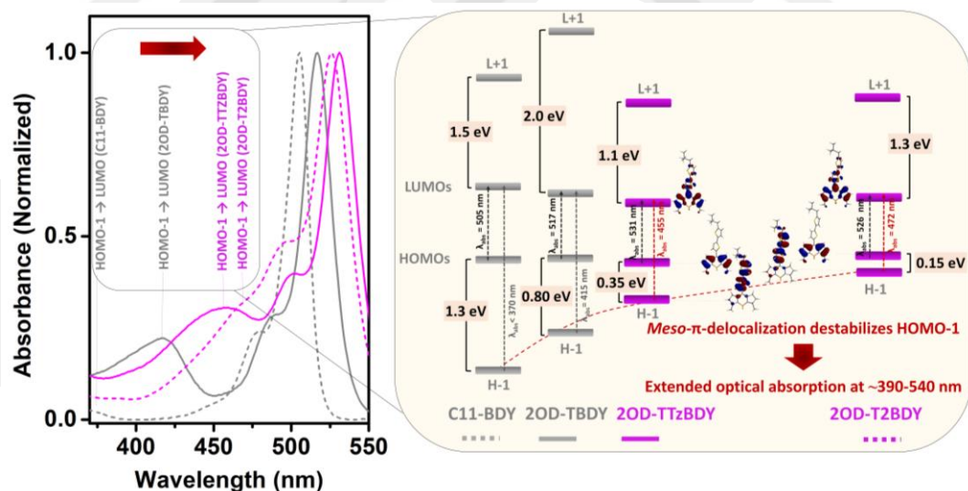
Figure 4.34 Optical absorption spectra of C11-BDY , 2OD-TBDY , 2OD-T2BDY , and 2OD-TTzBDY in dichloromethane ( 1.0 \times 10^{-5} M) showing higher energy optical transitions in the ~390-540 nm spectral region next to the main \pi \rightarrow \pi^* transitions, and the corresponding HOMO-1 , HOMO , LUMO , and LUMO+1 molecular orbital energies and wave function topographies (B3LYP/6-31G** level of theory). The red dashed line is a guide to the eye to illustrate the HOMO-1 destabilization for C11-BDY \rightarrow 2OD-TBDY \rightarrow 2OD-TTzBDY \rightarrow 2OD-T2BDY .
