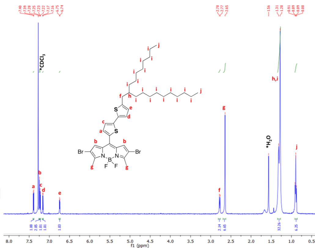
Figure 4.8 1 H NMR spectrum of 2OD-T2BDY-Br 2 in CDCl 3 at room temperature. CDCl 3 and H 2 O peaks originating from the NMR-solvent are denoted by asterisks.
