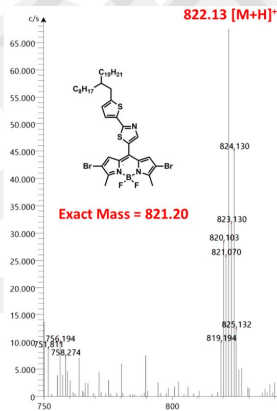
Figure 4.21 Positive ion mass spectrum of 2OD-TTzBDY-Br 2 measured via atmospheric pressure chemical ionization (MS-APCI).
