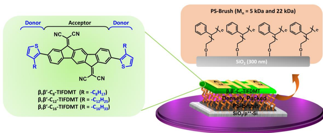
Figure 3.1 The chemical structures of solution-processable low-LUMO 2,2'-(2,8-bis(3-alkylthiophen-2-yl)indeno[1,2- b ]fluorene-6,12-diylidene)dimalononitrile small molecules, \beta,\beta' -C n -TIFDMT , having varied alkyl chain lengths ( n = 8, 12, 16), and the OFET device architecture employed in this study showing PS-brush ( M n = 5 kDa and 22 kDa)-based semiconductor-dielectric polymer interlayer.
