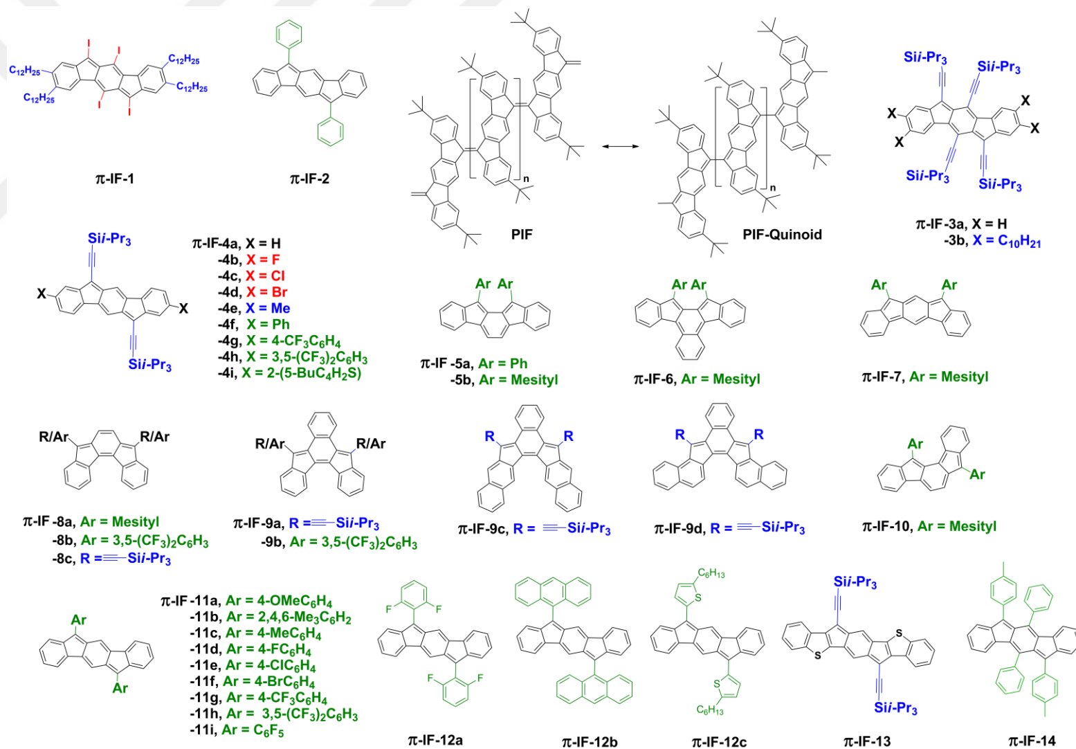
Figure 2.21 Chemical structures of fully conjugated indenofluorene ( \pi -IFs)-based semiconductors \pi -IFs-1-14 and PIF/PIF-Quinoid.
