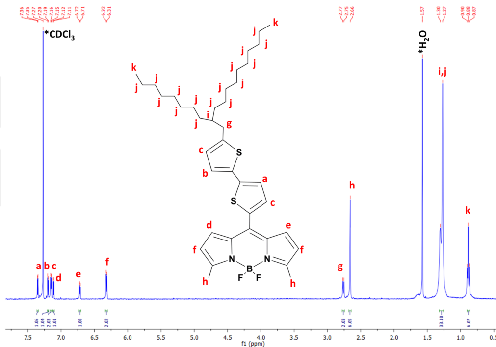
Figure 4.5 ^1\text{H} NMR spectrum of 2OD-T2BDY in \text{CDCl}_3 at room temperature. \text{CDCl}_3 and \text{H}_2\text{O} peaks originating from the NMR-solvent are denoted by asterisks.
