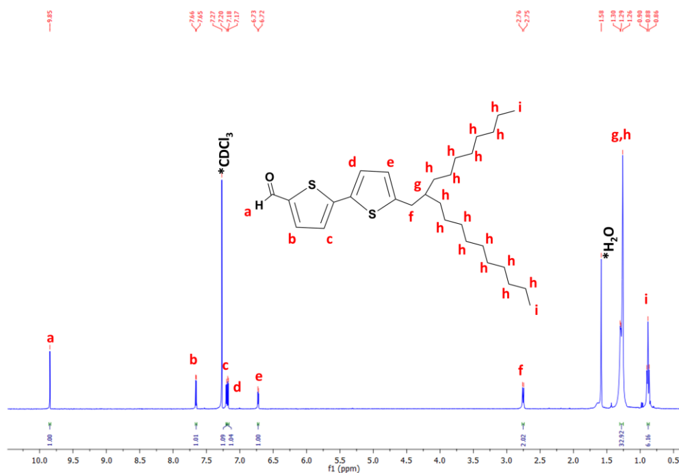
Figure 4.4 ^1\text{H} NMR spectrum of 2OD-T2-COH in \text{CDCl}_3 at room temperature. \text{CDCl}_3 and \text{H}_2\text{O} peaks originating from the NMR-solvent are denoted by asterisks.
