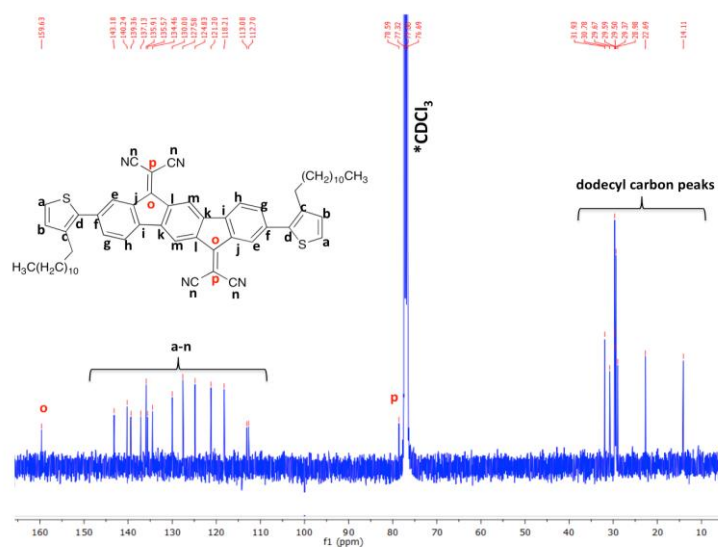
Figure 3.18 ^{13}\text{C} NMR spectra of \beta,\beta' -C12-TIFDMT in \text{CDCl}_3 at room temperature. (Bruker 400/Erciyes University-TAUM). ( \text{CDCl}_3 peak in NMR solvent is denoted by asterisks).
