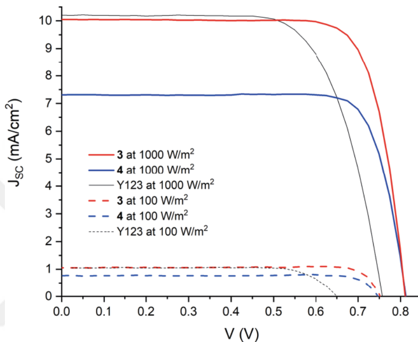
Figure 2.19 Current density ( J_{sc} ) vs. applied potential (V) curves of DSSCs (using I^-/I_3^- based electrolyte) fabricated with IF-TTF-1a (4 in the figure) and IF-TTF-1b (3 in the figure) dyes in comparison to a well-known dye Y123 without the IF \pi -core under 'AM1.5G illumination [92]. Reprinted with permission from reference 92. Copyright 2020, Wiley-VCH.
