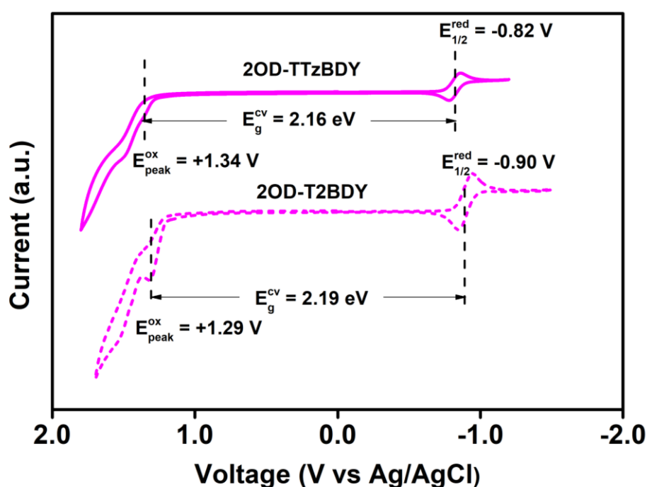
Figure 4.35 Full-range cyclic voltammograms of the meso- \pi -extended BODIPY acceptor building blocks 2OD-T2BDY and 2OD-TTzBDY in 0.1 M TBAPF 6 dichloromethane solution versus Ag/AgCl (3.0 M NaCl) at a scan rate of 100 mV s -1 .
