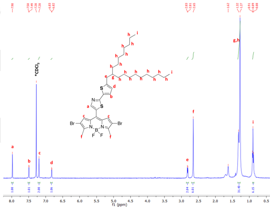
Figure 4.19 ^1\text{H} NMR spectrum of 2OD-TTzBDY-Br 2 in \text{CDCl}_3 at room temperature. \text{CDCl}_3 and \text{H}_2\text{O} peaks originating from the NMR-solvent are denoted by asterisks.
