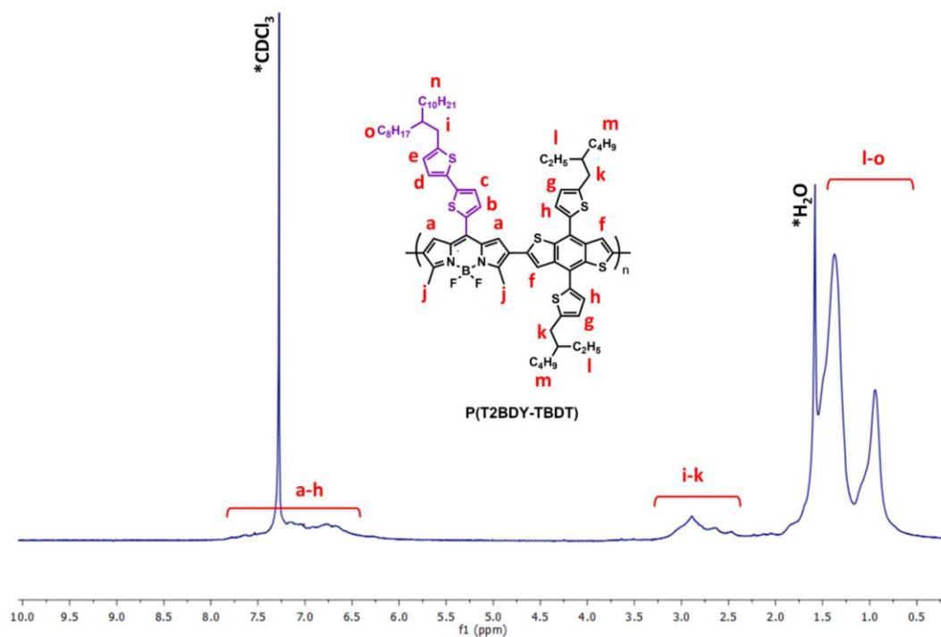
Figure 4.25 ^1\text{H} NMR spectrum of \text{P}(\text{T2BDY-TBDT}) in \text{CDCl}_3 at room temperature. \text{CDCl}_3 and \text{H}_2\text{O} peaks originating from the NMR-solvent are denoted by asterisks.
