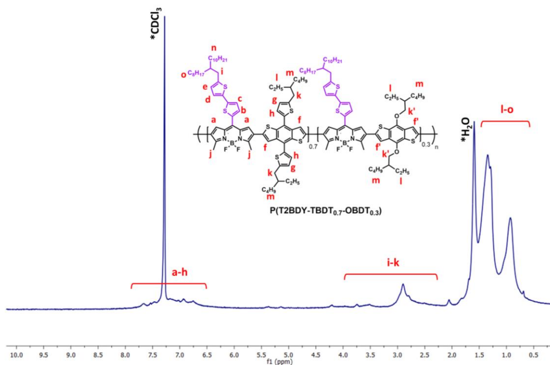
Figure 4.27 ^1H NMR spectrum of P(T2BDY-TBDT_{0.7}-OBDT_{0.3}) in CDCl_3 at room temperature. CDCl_3 and H_2O peaks originating from the NMR-solvent are denoted by asterisks.
