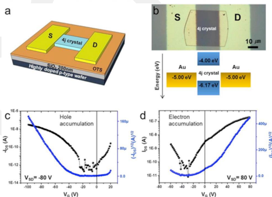
Figure 2.27 (a) Illustration of an OFET device with an active channel composed of a \pi -IF-11i (4j in the figure) single crystal. (b) Top-view optical micrograph of an OFET and the energy level diagram for Au/ \pi -IF-11i crystal/Au (bottom). (c, d) I – V transfer curves of OFETs with (c) negative and (d) positive drain voltages [133]. Reprinted with permission from reference 133. Copyright 2012, American Chemical Society.
