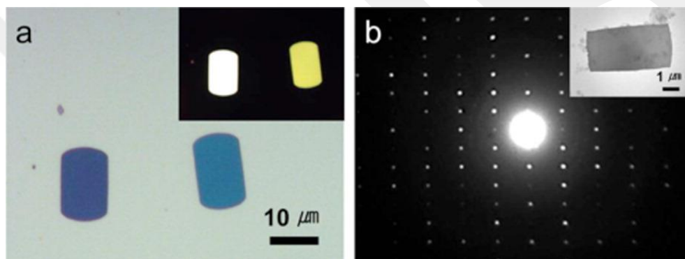
Figure 2.26 (a) Optical micrographs (OMs) of the single crystals of \pi -IF-11i from a solvent-exchange method. The inset displays an OM with crossed polarizers. (b) SAED pattern and (inset) bright-field TEM image of a single crystal of \pi -IF-11i [133]. Reprinted with permission from reference 133. Copyright 2012, American Chemical Society.
