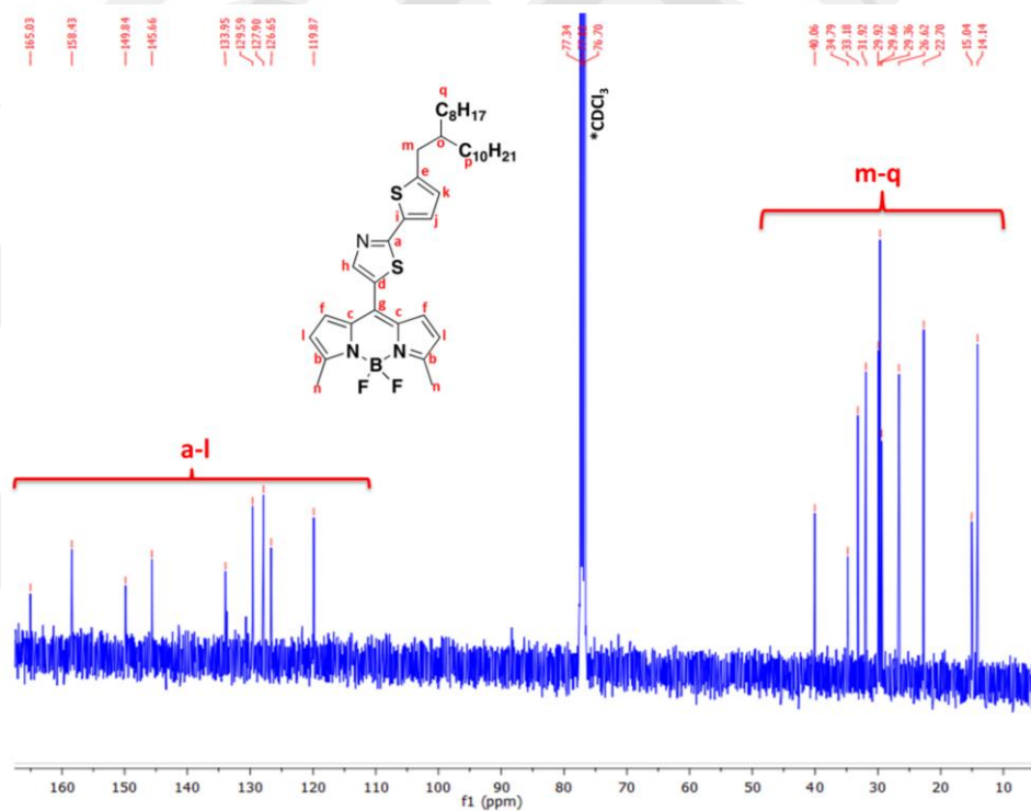
Figure 4.17 ^{13}\text{C} NMR spectrum of 2OD-TTzBDY in \text{CDCl}_3 at room temperature. \text{CDCl}_3 peak originating from the NMR-solvent is denoted by asterisk.
