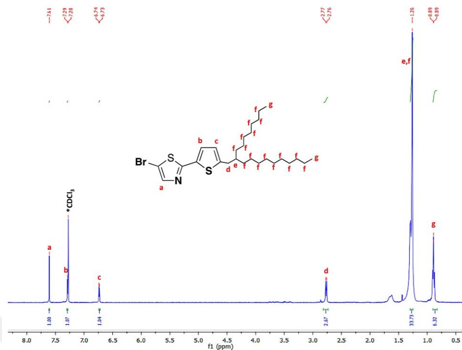
Figure 4.14 1 H NMR spectrum of 4 in CDCl 3 at room temperature. CDCl 3 peak originating from the NMR-solvent is denoted by asterisk.
