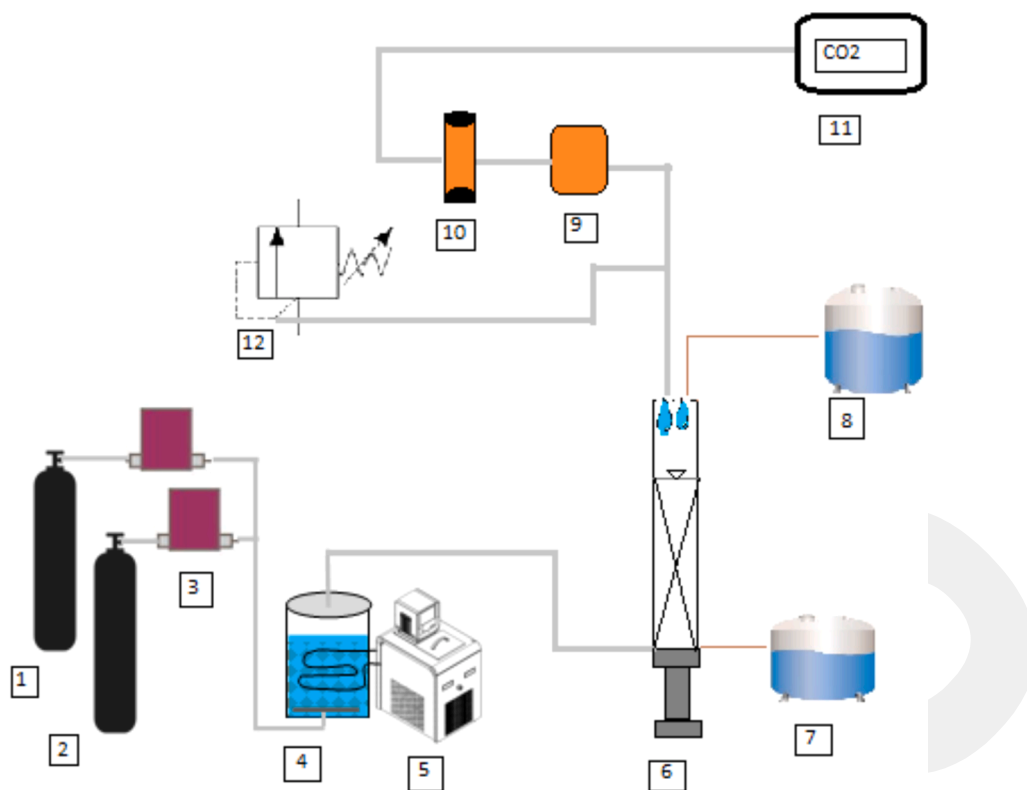
Fig. 3. The experimental setup: 1: CO 2 cylinder, 2: N 2 cylinder, 3: Mass flow controller, 4: Humidifier, 5: Heat exchanger, 6: Column, 7: Waste tank, 8: Solvent tank, 9: Dehumidifier gas regulator, 10: Dehumidifier, 11: CO 2 Analyzer (10.000-100.000ppm), 12: Relief valve.
