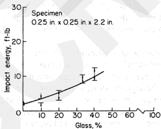
Figure 1.5 Influence of Adding Glass Fibers in a Graphite-Epoxy Laminate regarding Impact Energy [4]
