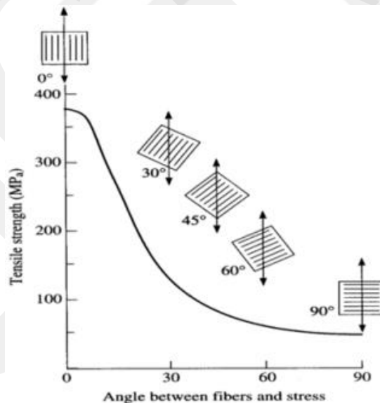
Figure 1.3 Fiber Angle and Tensile Strength Relation [14]
