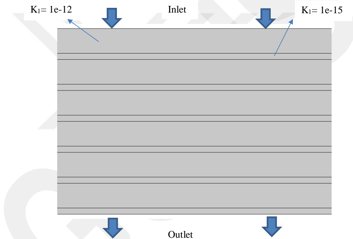
Figure 5.10 Geometry of Heterogeneous Staggered Layers Geometry for Simulation 6
