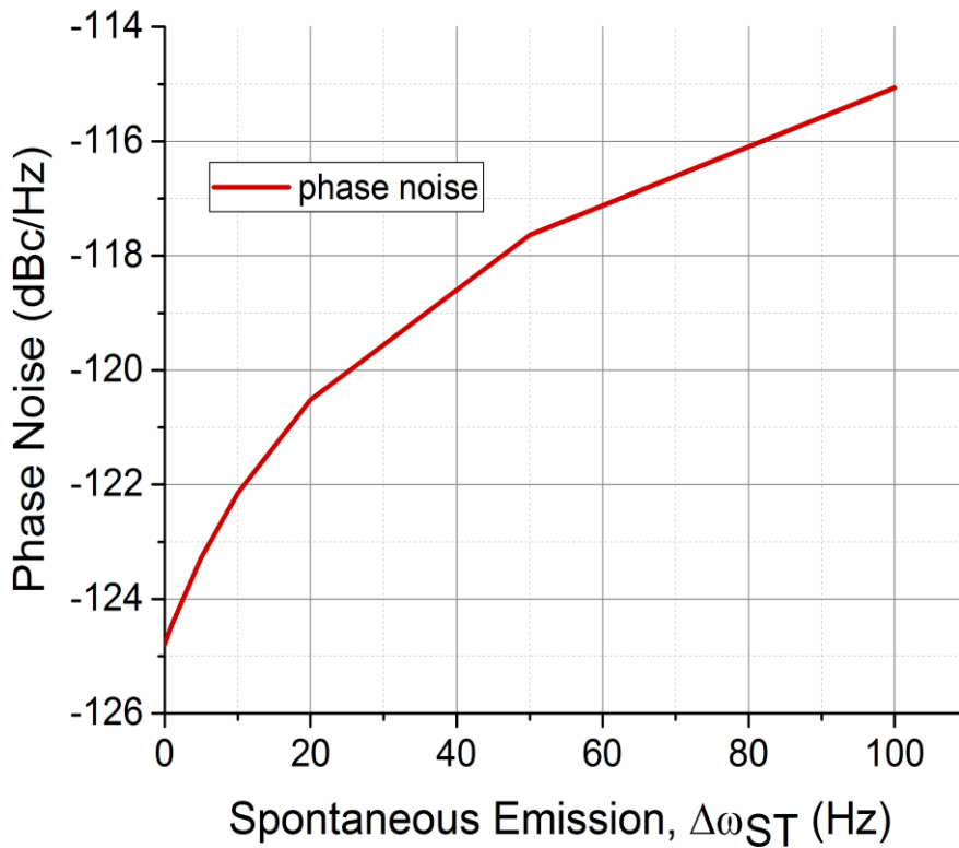
Figure 4.2.2; Phase noise versus spontaneous emission, ( \Delta\omega_{ST} ) at 1 MHz offset and assuming 0 Hz frequency mismatch, \Delta\omega_{ST}
