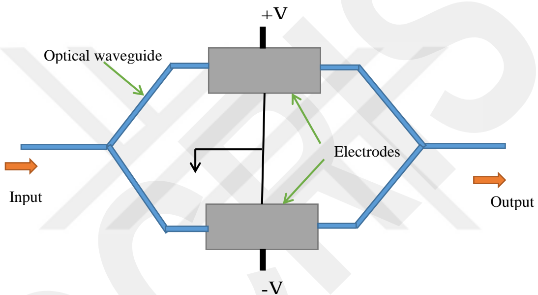
Figure 3.1.1.4 Mach-Zehnder interferometer based electro-optic modulator
