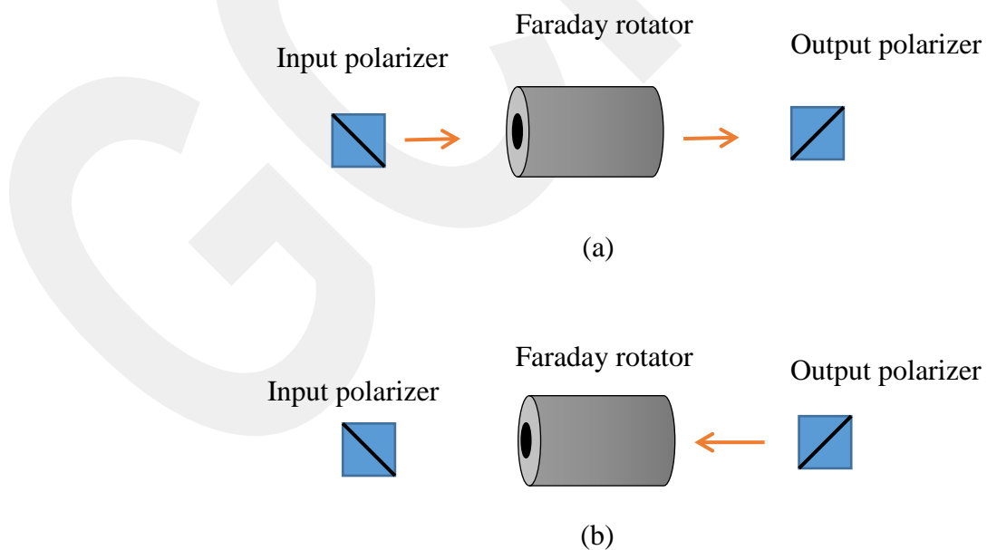
Figure 3.1.1.5; Optical Isolator with light passing from left (a) and blocked from right (b)
