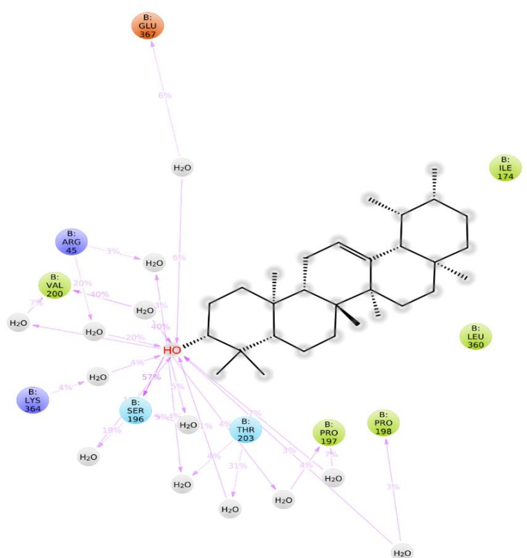
Figure 4. Analysis of the way \alpha -amyryn interacts with viral DNA-directed RNA polymerase indicated that the macromolecular residues shown in green had hydrophobic connections, and the sky blue residues had polar connections with the complexed ligand. The orange-colored residues were negative, and the dark blue were positive.
