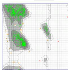
Figure 1. Ramachandran plot for the structural model of DNA-directed RNA polymerase of monkeypox virus.
