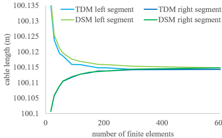
Fig. 7. Segment cable lengths vs. number of finite elements.
