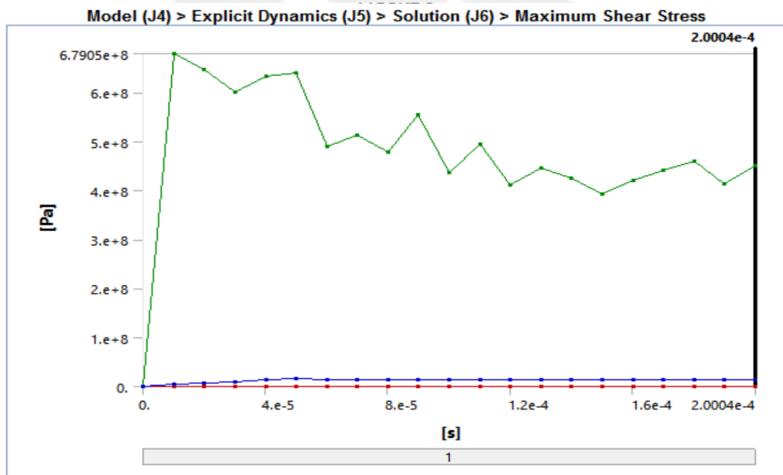
In addition to that, for a clear comprehension, the graph below is plotted with the values shown, green line representing the maximum shear stress, red line representing minimum and blue line representing average shear stress.
