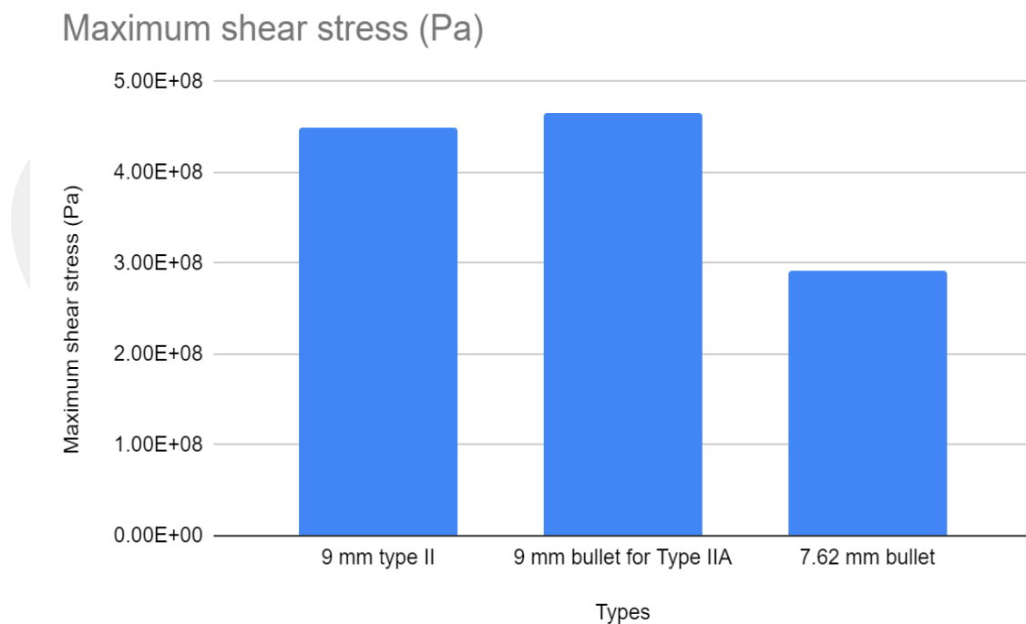
Figure 4.60 Maximum shear stress results chart providing a comparison for all tested projectiles
