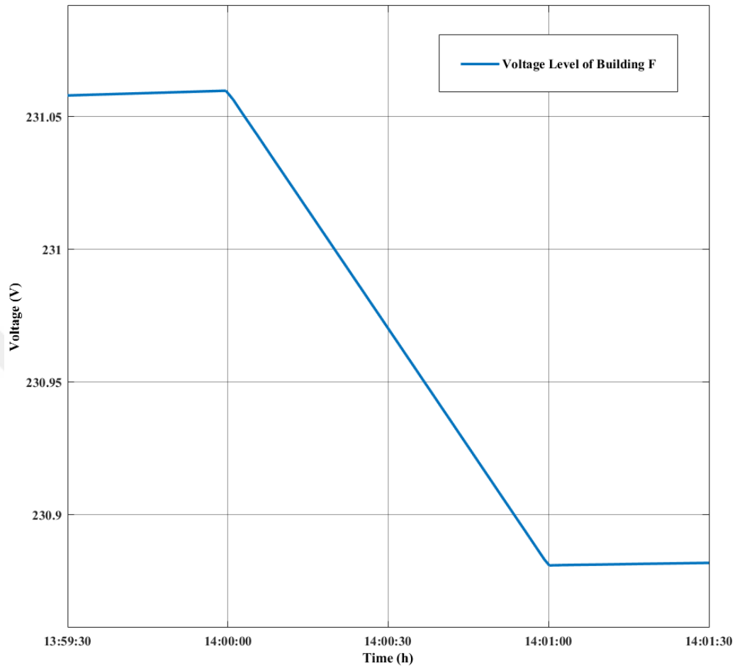
Figure 4.3.3.2.5 60% PV Penetration voltage graph of Building F with BSS
