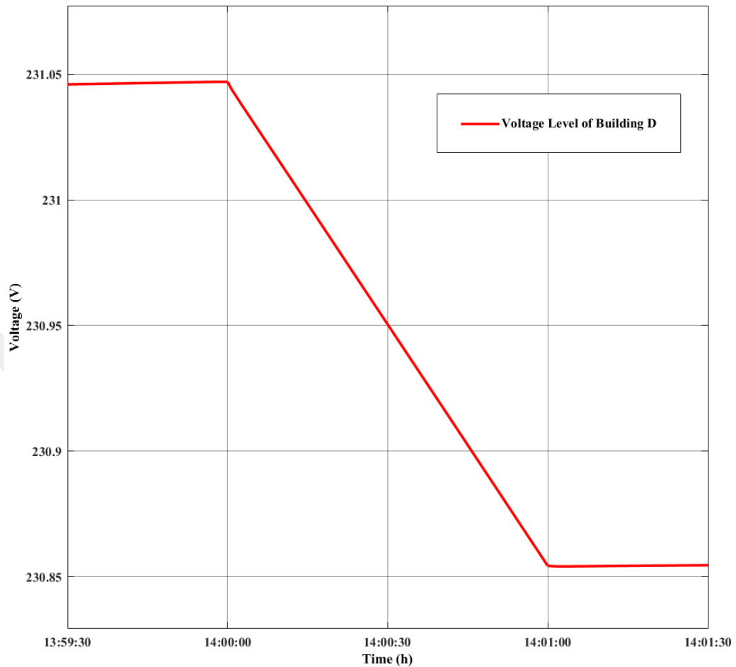
Figure 4.3.3.3.4 40% PV Penetration voltage graph of Building D with BSS
