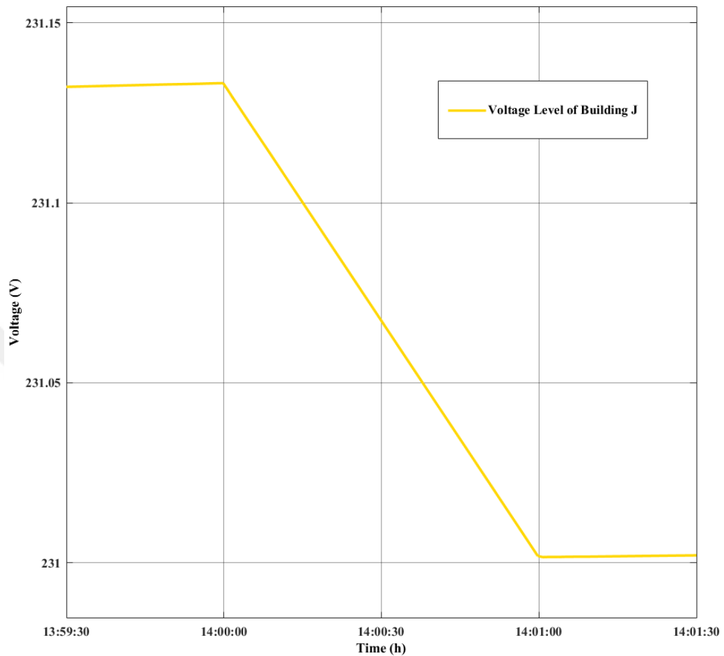
Figure 4.3.3.2.3 60% PV Penetration voltage graph of Building J without BSS
