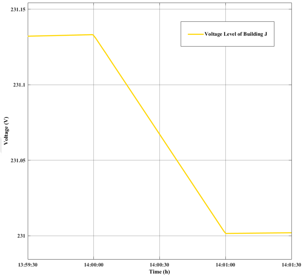
Figure 4.3.3.2.6 60% PV Penetration voltage graph of Building J with BSS
