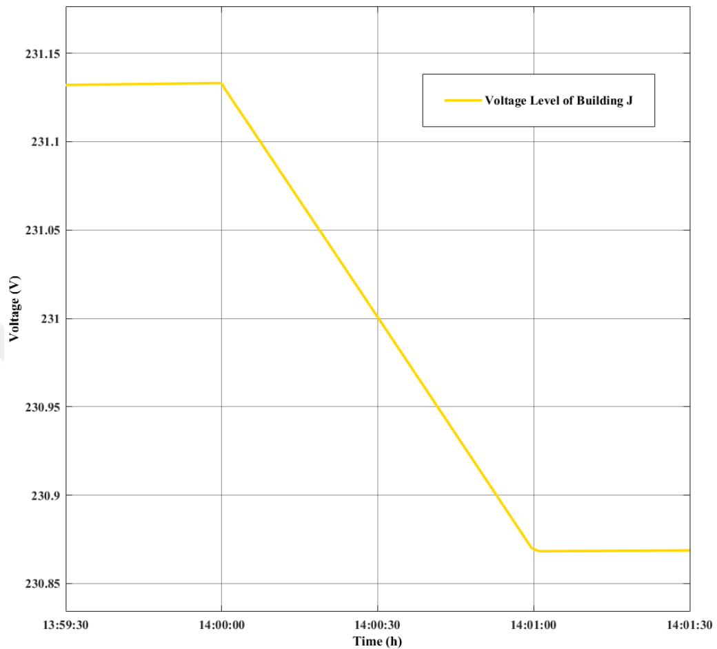
Figure 4.3.3.4.6 20% PV Penetration voltage graph of Building J with BSS
