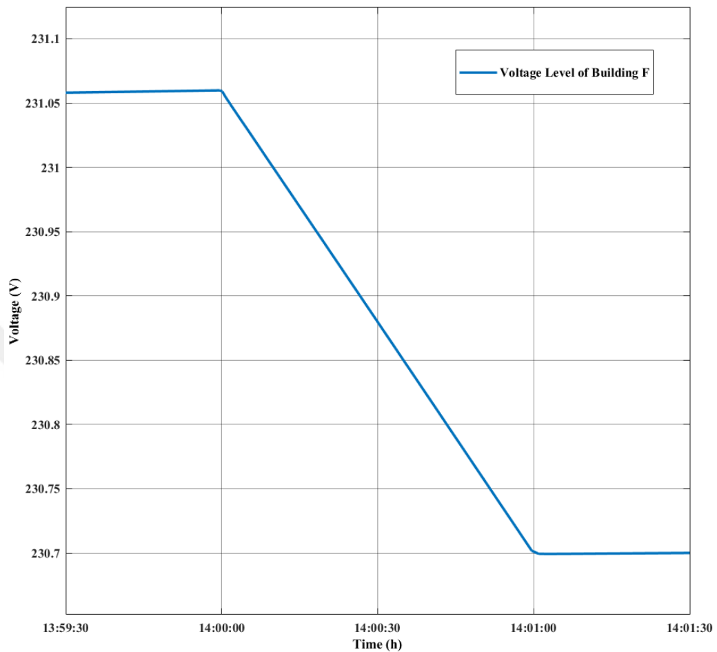
Figure 4.3.3.4.5 20% PV Penetration voltage graph of Building F with BSS
