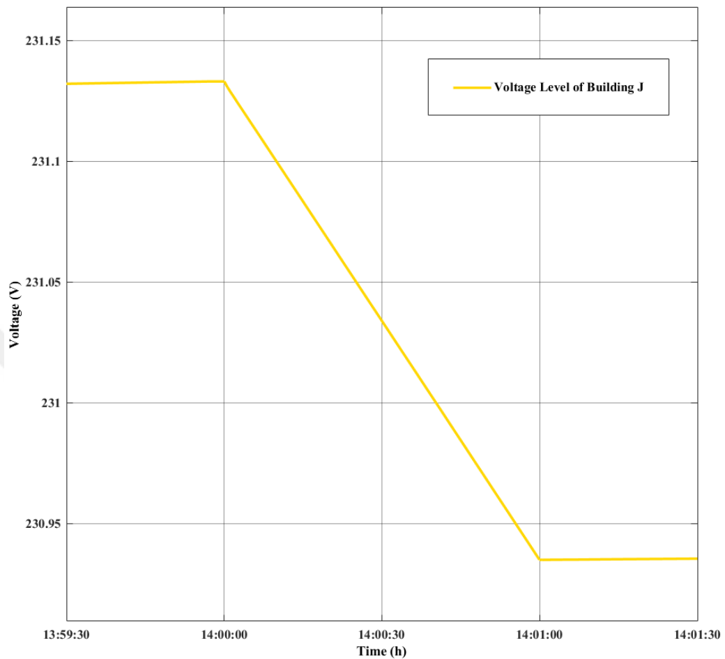
Figure 4.3.3.3.6 40% PV Penetration voltage graph of Building J with BSS
