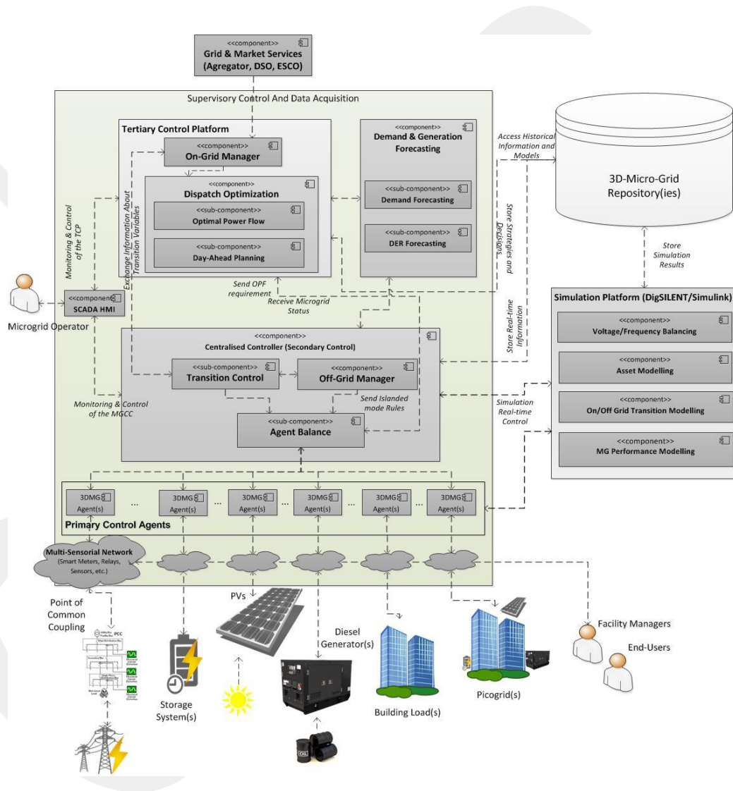
Figure 3.3.1 3DMicroGrid system architecture
