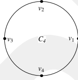
Figure 4: Circle graph with 4 vertices
