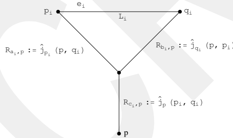
Figure 2: Circuit reduction of \Gamma with reference to an edge e_i and a point p .
