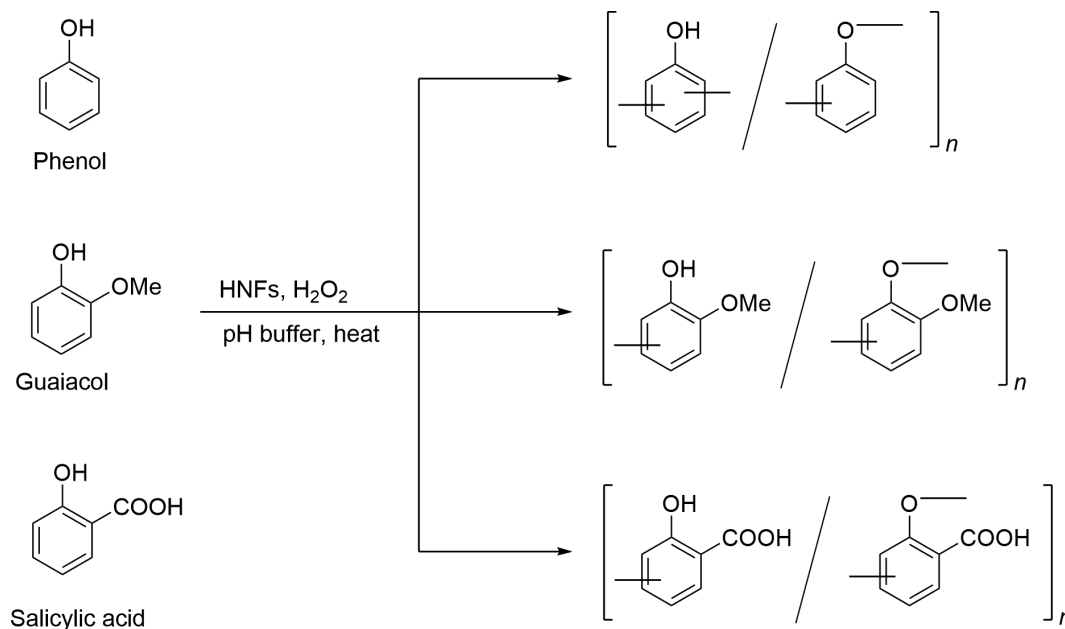
FIGURE 1 Polymerization of phenol derivatives by HNFs and \text{H}_2\text{O}_2 , and the possible polymeric structures. HNFs: hibrit nanoflowers (green tea- \text{Cu}^{2+} , caffeine- \text{Cu}^{2+} , or catechin- \text{Cu}^{2+} ).
