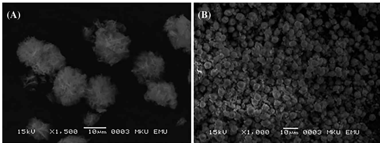
FIGURE 5 SEM images of caffeine- \text{Cu}^{2+} (A) and catechin- \text{Cu}^{2+} (B) nanobiocatalysts.
