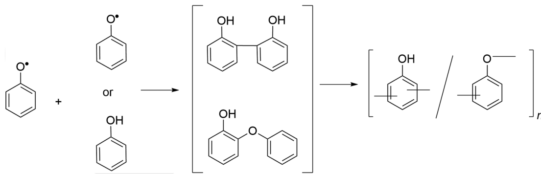
FIGURE 6 The polymerization mechanism of phenol.
