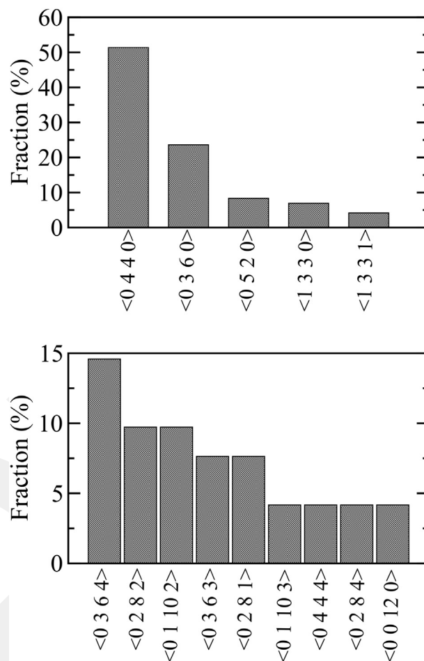
Fig. 4. Fraction of Si- and Mg-centered Voronoi polyhedrons. Polyhedrons having a fraction of less than 4% are not shown in the figure.
