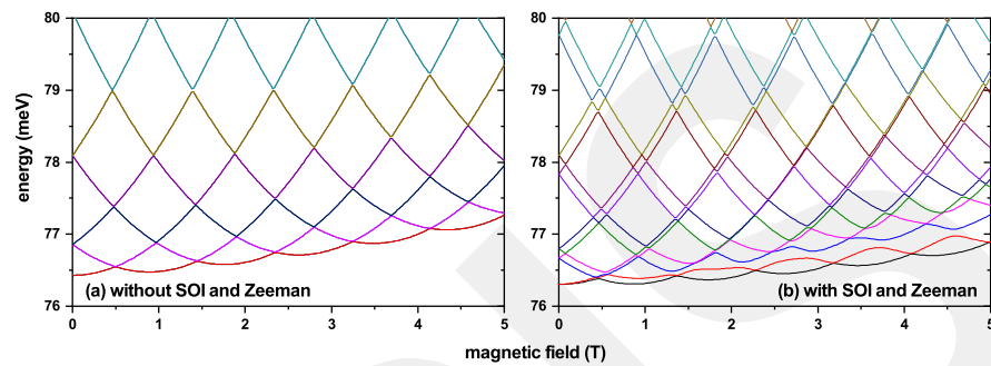
Figure 2. Electron energy in a double GaAs-Al 0.3 Ga 0.7 As quantum ring as a function of a magnetic field without (a) and with (b) SOI and Zeeman effects.
