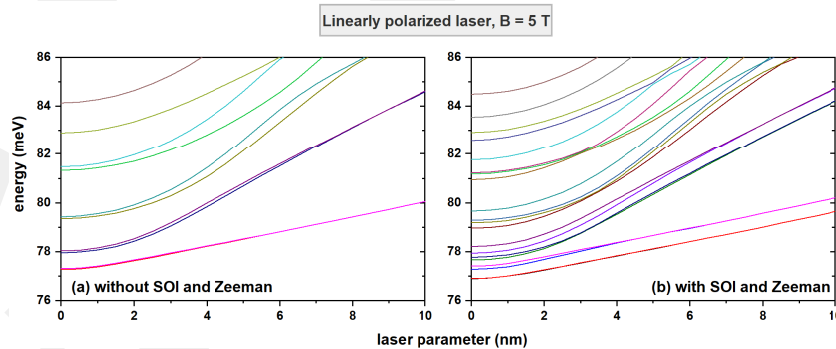
Figure 4. Comparative behavior of electron energy levels in a double GaAs-Al 0.3 Ga 0.7 As quantum ring as a function of the linearly polarized intense laser field parameter \alpha_0 in the presence of a magnetic field and for two different cases: (a) without SOI and Zeeman and (b) with SOI and Zeeman.
