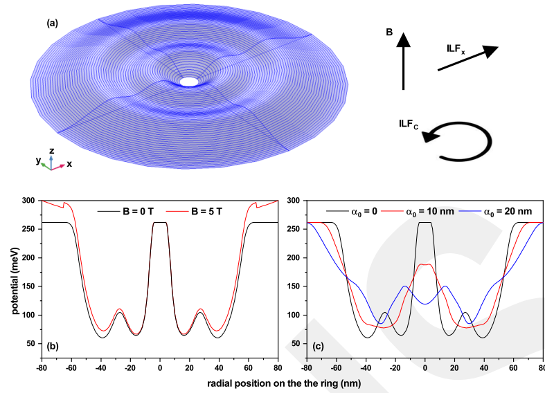
Figure 1. (a) Schematic representation of a double GaAs-Al 0.3 Ga 0.7 As quantum ring, with the profile taken from the work of Kuroda et al. [19]. The drawn vectors represent a magnetic field B in the z -direction, a nonresonant intense laser field for x , and circular polarizations. (b) Confinement potential with and without the presence of a magnetic field. (c) Laser-dressed potential for the three values of laser parameter \alpha_0 .
