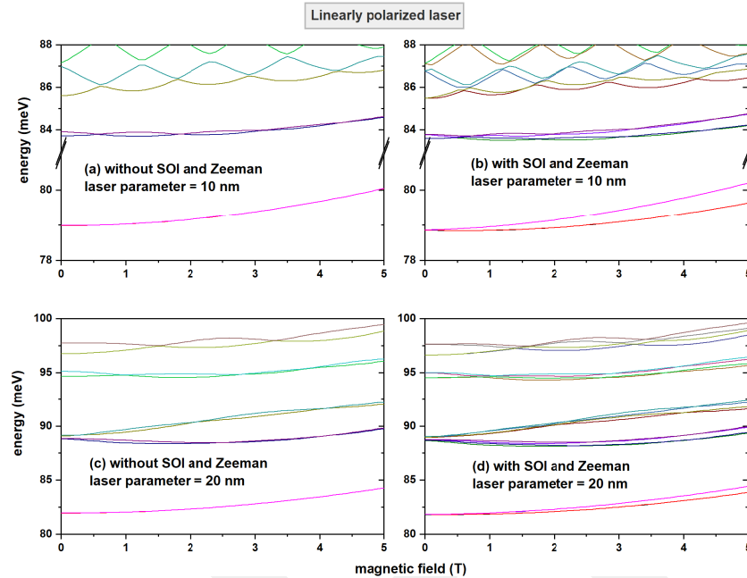
Figure 3. Electron energy in a double GaAs-Al 0.3 Ga 0.7 As quantum ring as a function of magnetic field and under the presence of a linearly x polarized intense laser field (ILF) for two laser parameter values: \alpha_0 : 10 nm and 20 nm.
