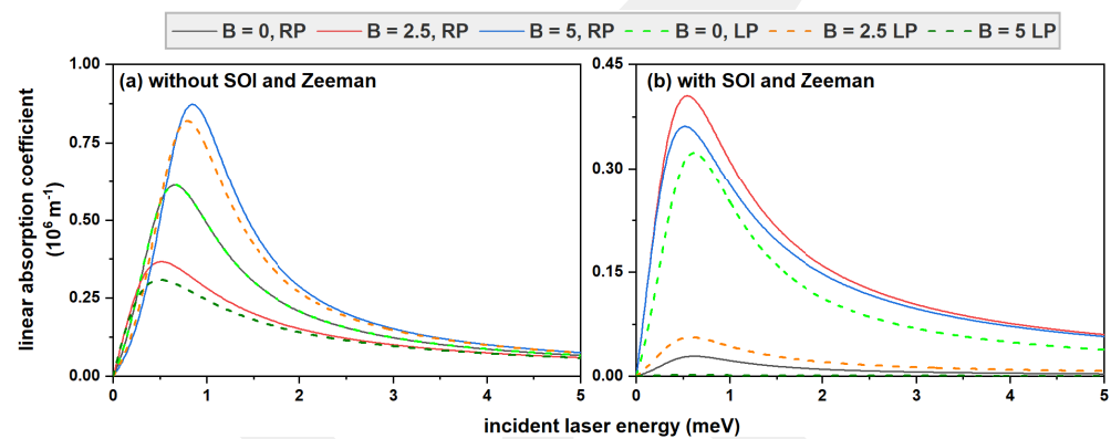
Figure 7. Linear absorption coefficient as a function of incident laser energy in a double GaAs-Al 0.3 Ga 0.7 As quantum ring for three values of the magnetic field: B = 0, 2.5 , and 5 T. Panel (a) does not include the spin interactions, whereas in (b), it is added. The solid and dashed lines correspond to right and left circular laser polarizations, respectively.
