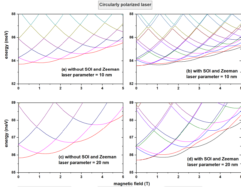
Figure 5. Electron energy in a double GaAs-Al 0.3 Ga 0.7 As quantum ring as a function of magnetic field and under the presence of a circularly polarized intense laser field (ILF) for two laser parameter values: \alpha_0 : 10 nm (first line) and 20 nm (second line).
