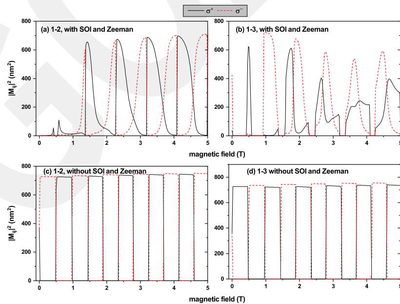
Figure 6. Squared matrix elements in a double GaAs-Al 0.3 Ga 0.7 As quantum ring as a function of magnetic field for right and left circularly polarized laser fields, \sigma^+ and \sigma^- , respectively. In panels (a,b), the SOI and Zeeman contributions are included; in contrast, for panels (c,d), the SOI and Zeeman contributions are turned off. For both conditions, the transitions 1–2 and 1–3 are studied.
