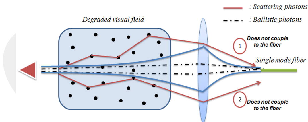
Figure 7. Receiver architecture with single mode fiber.
