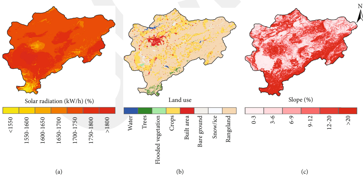
FIGURE 3: Solar radiation, land use, and slope maps of Kayseri.
