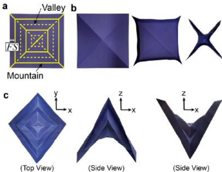
Figure 2.22 The general geometry of the hyper origami (Filipov & Redoutey, 2018)
