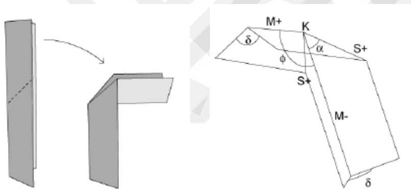
Figure 2.10 Illustration of the reverse fold (Buri & Weinand, 2010)
