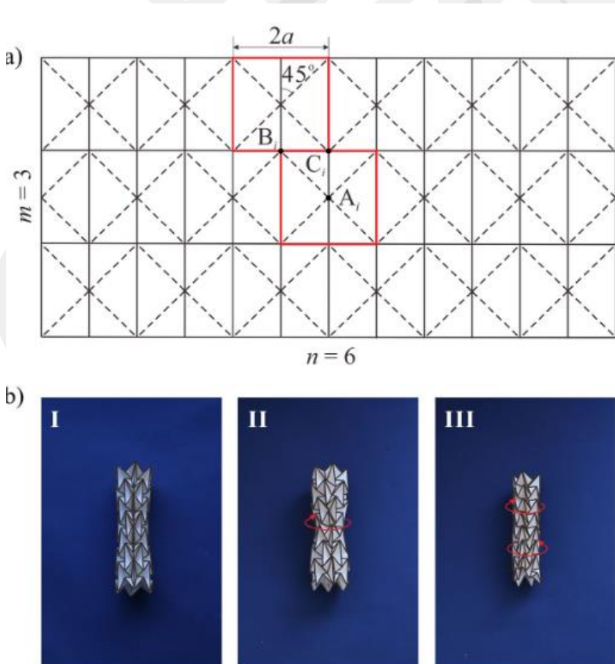
Figure 2.21 Waterbomb crease pattern and 3D visuals (Feng et al., 2018)
