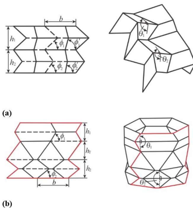
Figure 2.33 Graded behavior drawing of Miura Ori (Xie et al., 2016)
