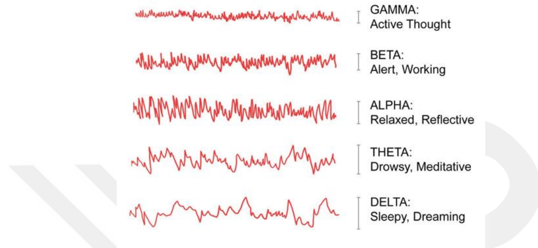
Figure 2.1.1 EEG frequency bands [3].
