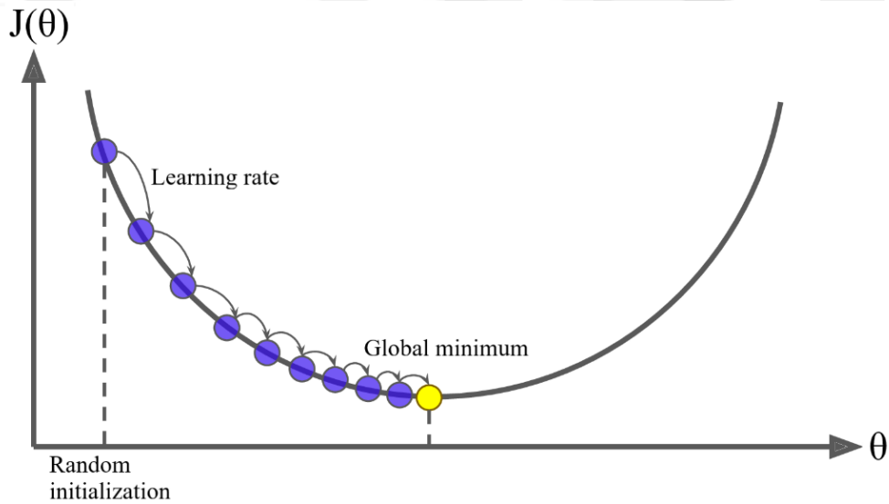
Figure 3.3 Visualization of the gradient descent optimizer
