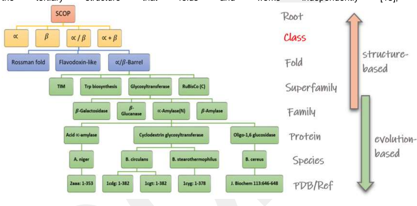
Figure 2. Part of the SCOP (version 1) Hierarchy [18].
