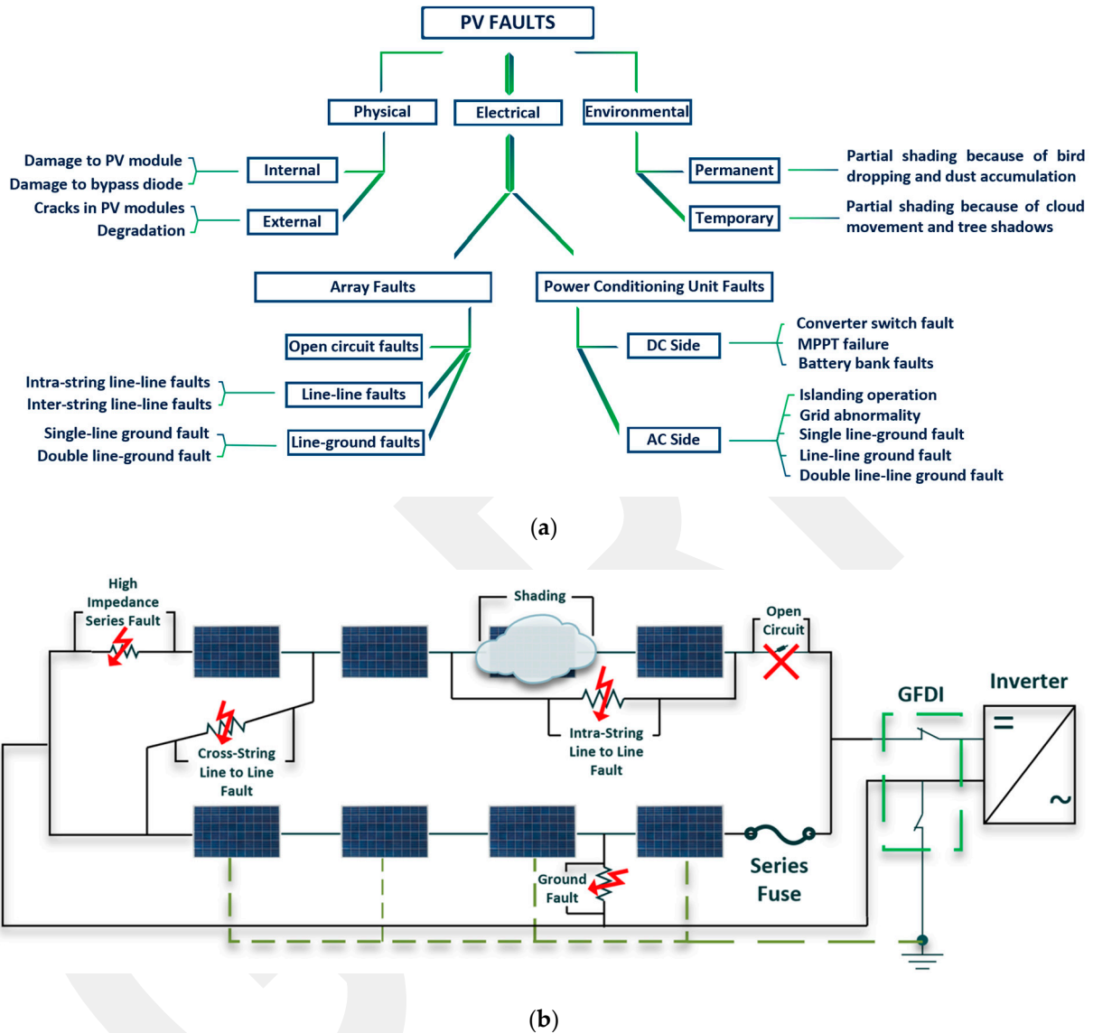
Figure 4. (a) Various faults on PV system; (b) Types of faults that can occur in PV system and the use of GFDI device.
