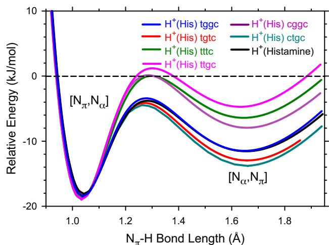
Fig. 2. Relaxed potential energy surfaces of H^+(\text{His}) and H^+(\text{histamine}) along the \text{N}_\pi\text{--H--N}_\alpha coordinate linking the [\text{N}_\pi, \text{N}_\alpha] (left side) and [\text{N}_\alpha, \text{N}_\pi] (right side) conformers calculated at the B3LYP/6-311+G(d,p) level. The energy zero is set to the zero point energy of the harmonic frequency in the [\text{N}_\pi, \text{N}_\alpha] potential well.
