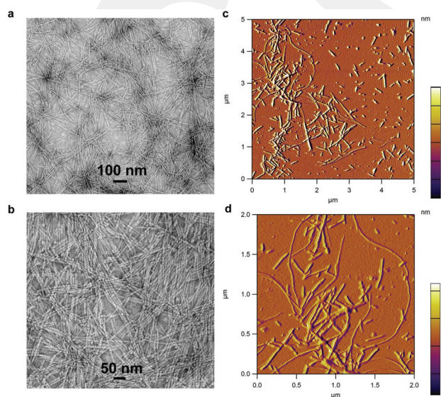
Fig. 5 Imaging of the C 8 -BTBT-peptide molecule. TEM (a and b) and AFM (c and d) images of the C 8 -BTBT-peptide nanofibers.
