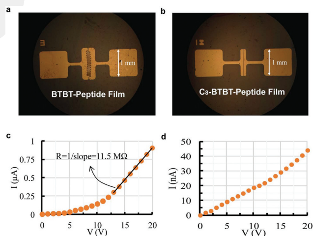
Fig. 6 Optical microscope images of Au contacts on the BTBT-peptide film with L = 20 \mu m and W = 4 mm (a) and the C 8 -BTBT-peptide film with L = 10 \mu m and W = 1 mm (b). I - V characteristics of the BTBT-peptide (c) and the C 8 -BTBT-peptide films between two Au electrodes (d).
