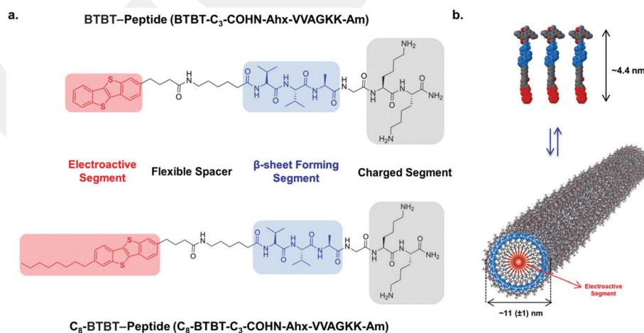
Fig. 1 (a) Molecular structures of the [1]benzothieno [3,2- b ] benzothiophene (BTBT)-peptide amphiphiles, the BTBT-peptide (BTBT-C 3 -COHN-Ahx-VVAGKK-Am) and the C 8 -BTBT-peptide (C 8 -BTBT-C 3 -COHN-Ahx-VVAGKK-Am). (b) A schematic presentation of the self-assembly process for the BTBT-peptide amphiphile showing the proposed nanofiber structure with the computed molecular length ( \sim 4.4 nm) and the measured nanofiber diameter ( \sim 11 \pm 1 nm).
