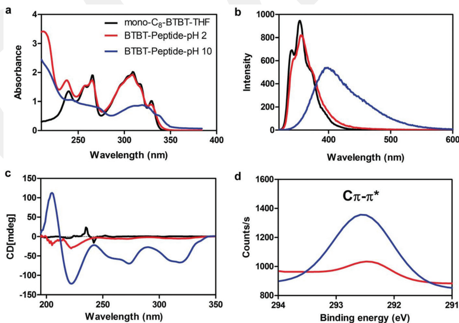
Fig. 2 Spectroscopic characterization of the BTBT-peptide self-assembly under different pH conditions. (a) UV-vis absorption, (b) fluorescence emission spectra ( \lambda_{ex} = 310 \text{ nm} ) and (c) CD spectrum. (d) The XPS spectrum of C 1s for BTBT-peptide films prepared at pH = 2 and pH = 10.
