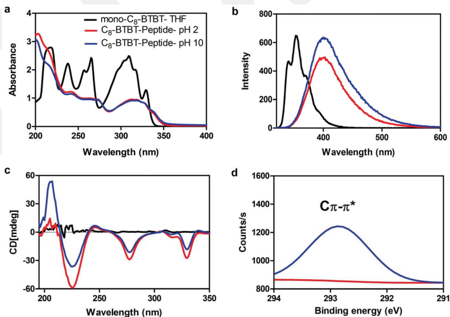
Fig. 4 Spectroscopic characterization of the C 8 -BTBT-peptide self-assembly under different pH conditions. (a) UV-vis absorption, (b) fluorescence emission spectra ( \lambda_{\text{ex}} = 310 nm) and (c) CD spectrum. (d) XPS spectrum of C 1s for the C 8 -BTBT-peptide films prepared at pH = 2 and pH = 10.
