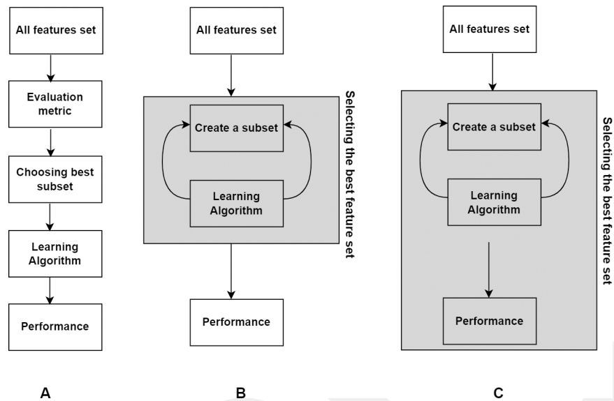
Figure 1 Three basic types of FS methods. (A) Filter. (B) Wrapper. (C) Embedded.
