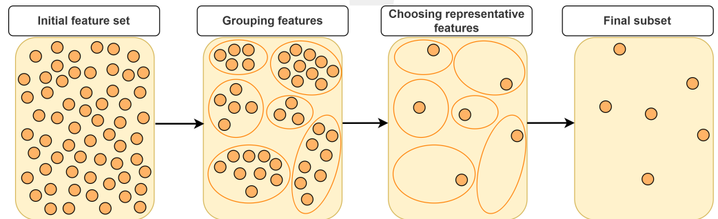
Figure 3 Typical approach for representative feature selection based on grouping.
