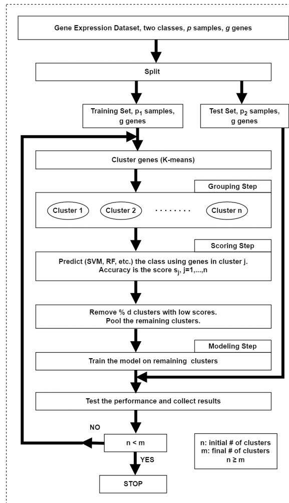
Figure 4 The workflow of the SVM-RCE algorithm. The grouping step for grouping genes into clusters, the scoring step for assigning score for each cluster and selecting significant clusters, the modeling step for training the model with top-ranked clusters.
