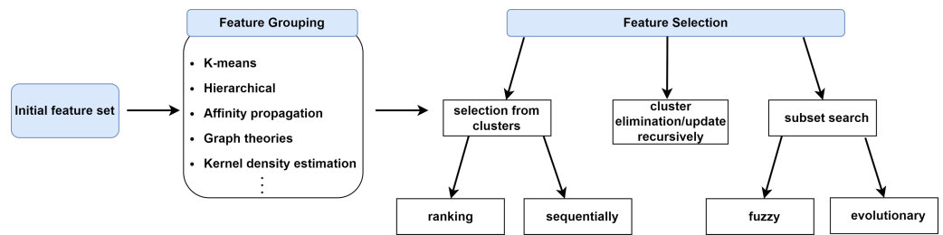
Figure 2 The representation of feature selection approaches based on grouping.
