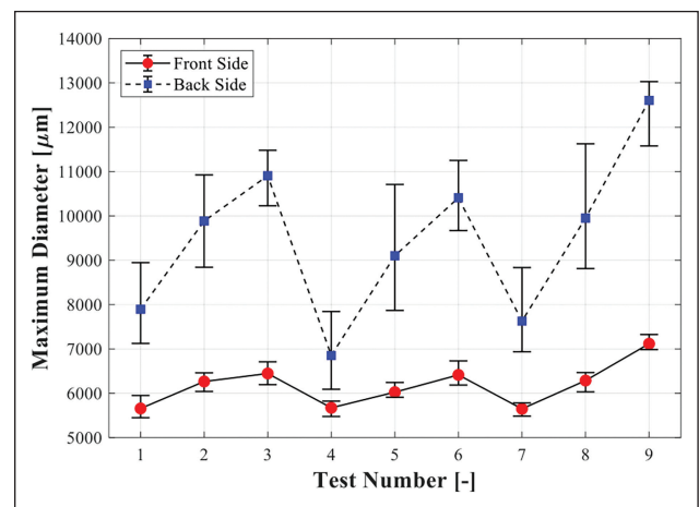
Figure 4. Maximum damaged size on the (a) front and (b) back sides of the composite plate.
