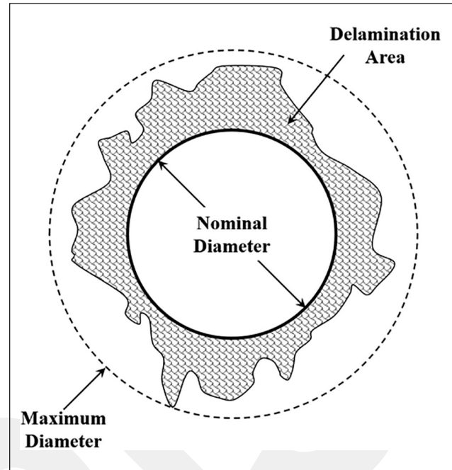
Figure 2. Calculation of delamination factor.
