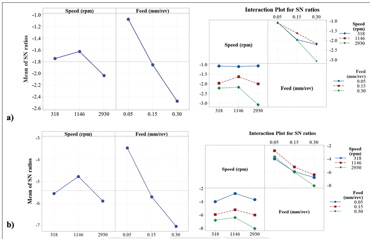
Figure 5. Effects of drilling parameters on the S/N ratio for the delamination factors on the (a) front and (b) back sides of the composite plate.
