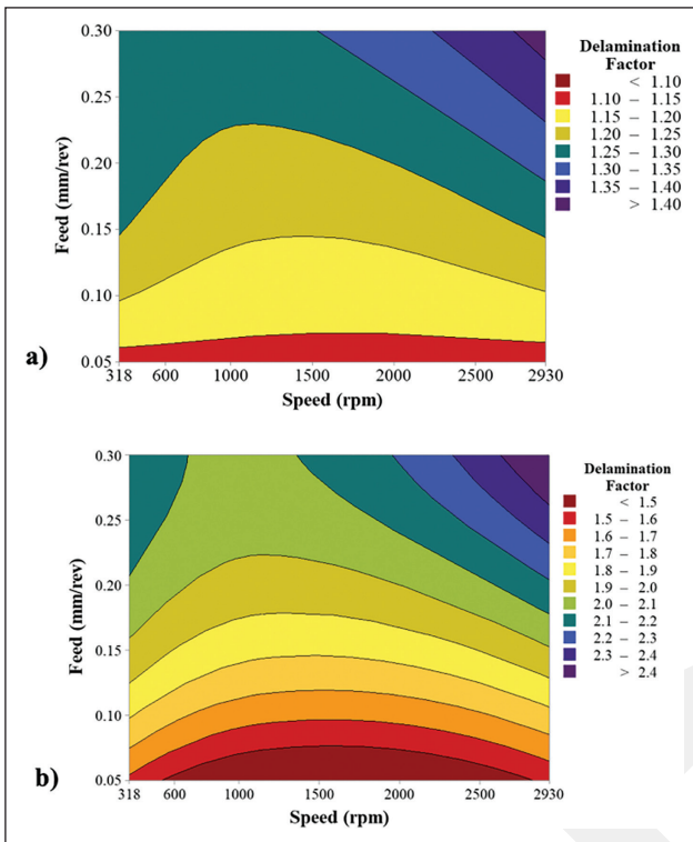
Figure 6. Delamination factor as a function of drilling parameters on the (a) front and (b) back sides of the composite plate.
