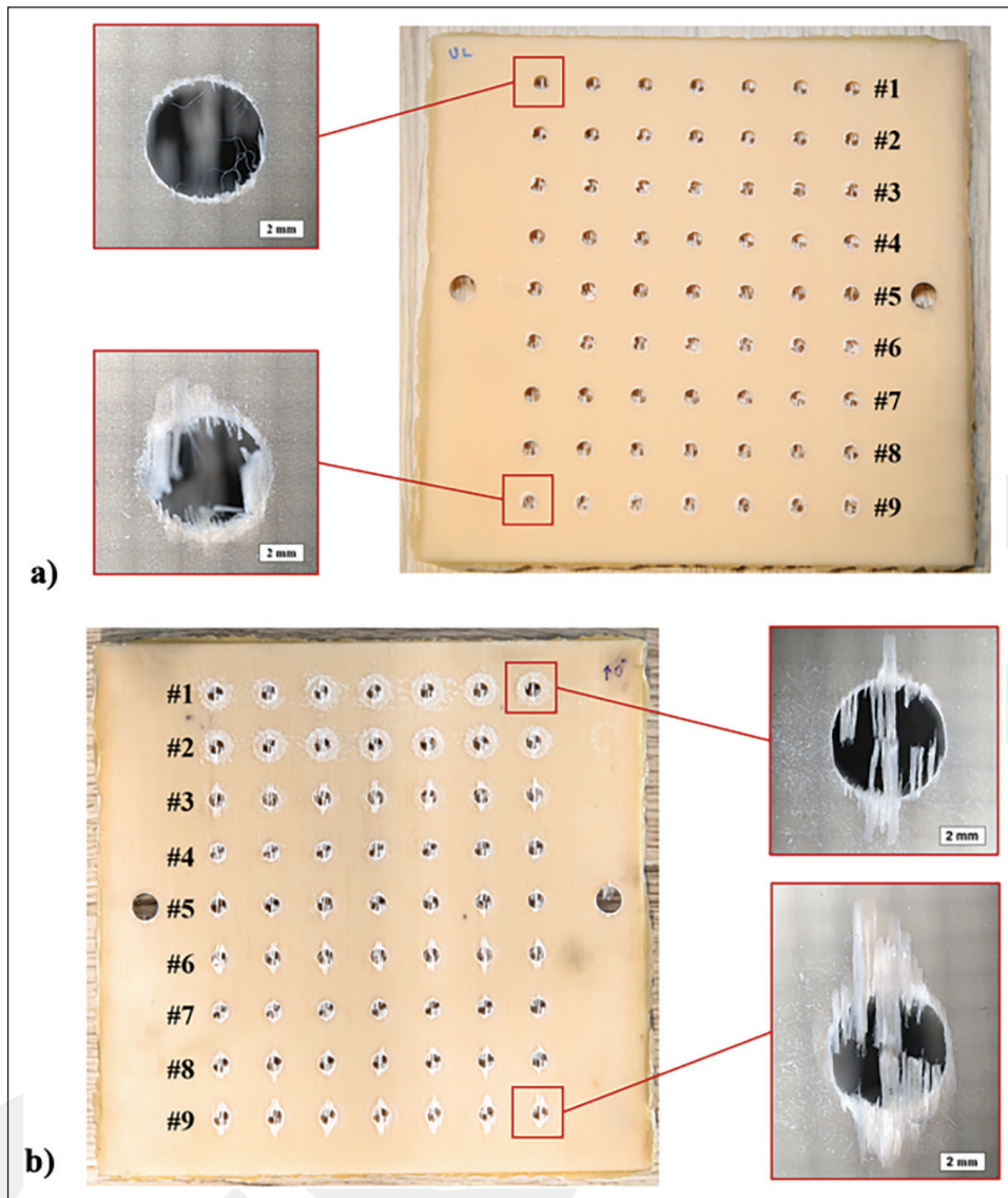
Figure 3. (a) Front and (b) back sides of the glass fiber reinforced composite plates after drilling tests.
