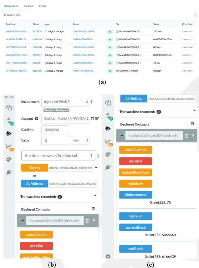
FIGURE 3. Proposed smart contract in Remix. (a) executed transactions in Ropsten Test Network, (b) deployment, and (c) running.
