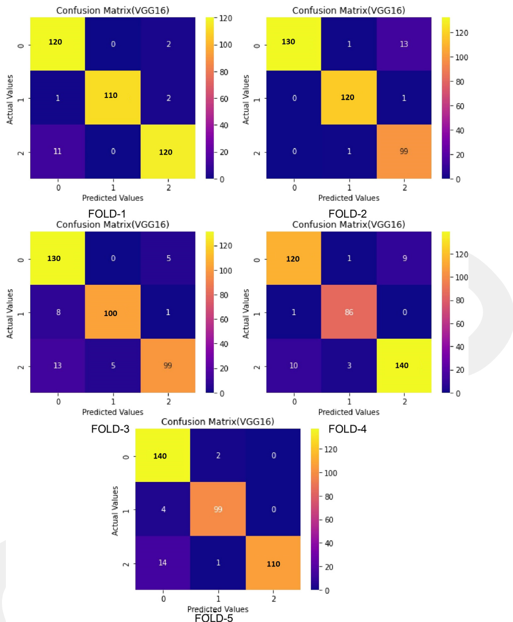
Fig. 7. Confusion Matrix:VGG16 on 5-Folds(0-Normal, 1-COVID19,2-Viral).
