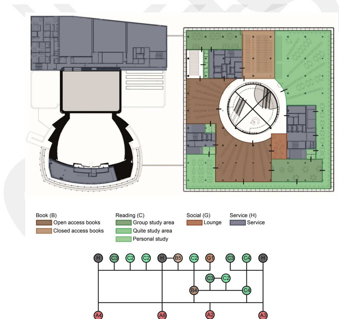
Figure 4.2.3. Library of Birmingham Second Floor and Its Syntactic Analysis (Plan scheme is re-produced from the drawings on https://www.mecanoo.nl/Projects/project/57/Library-of-Birmingham ) 10
