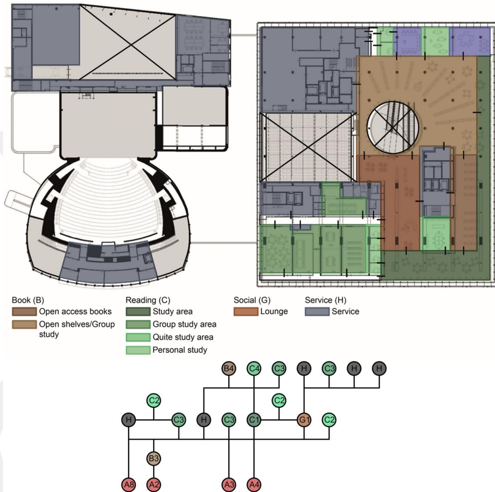
Figure 4.2.2. Library of Birmingham First Floor and Its Syntactic Analysis
