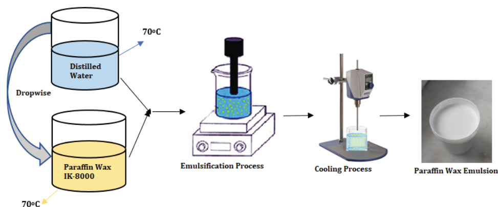
Figure 1. Flow Sheet of Paraffin Wax Emulsion Preparation.
