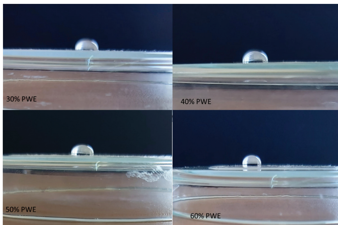
Figure 2. Images displaying water drops on glass surfaces coated by a different paraffin emulsion.
