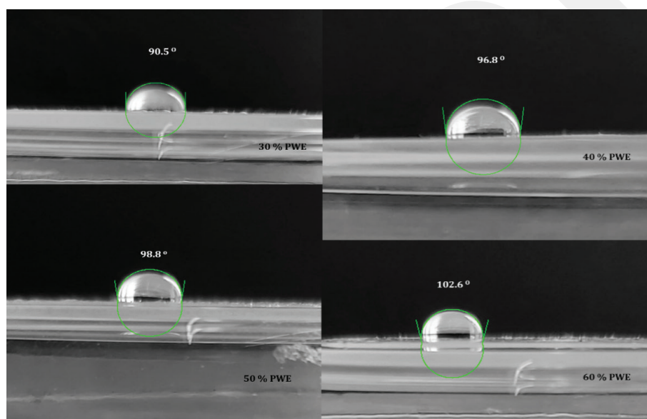
Figure 6. Results of contact angle measurements of; 30%wt. PWE, 40 %wt. PWE, 50%wt. PWE and 60%wt. PWE samples.
