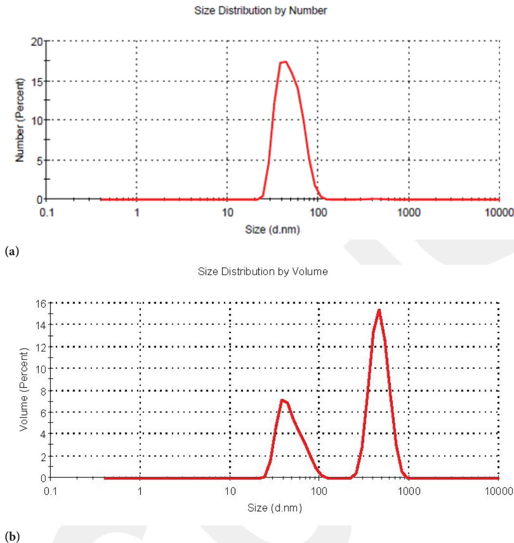
Figure 8. Particle size distribution (PSD) analysis result for the sample with 17.5 %wt. paraffin, 2.5 %wt. emulsifier, (a) number-based distribution, (b) volume-based distribution.
