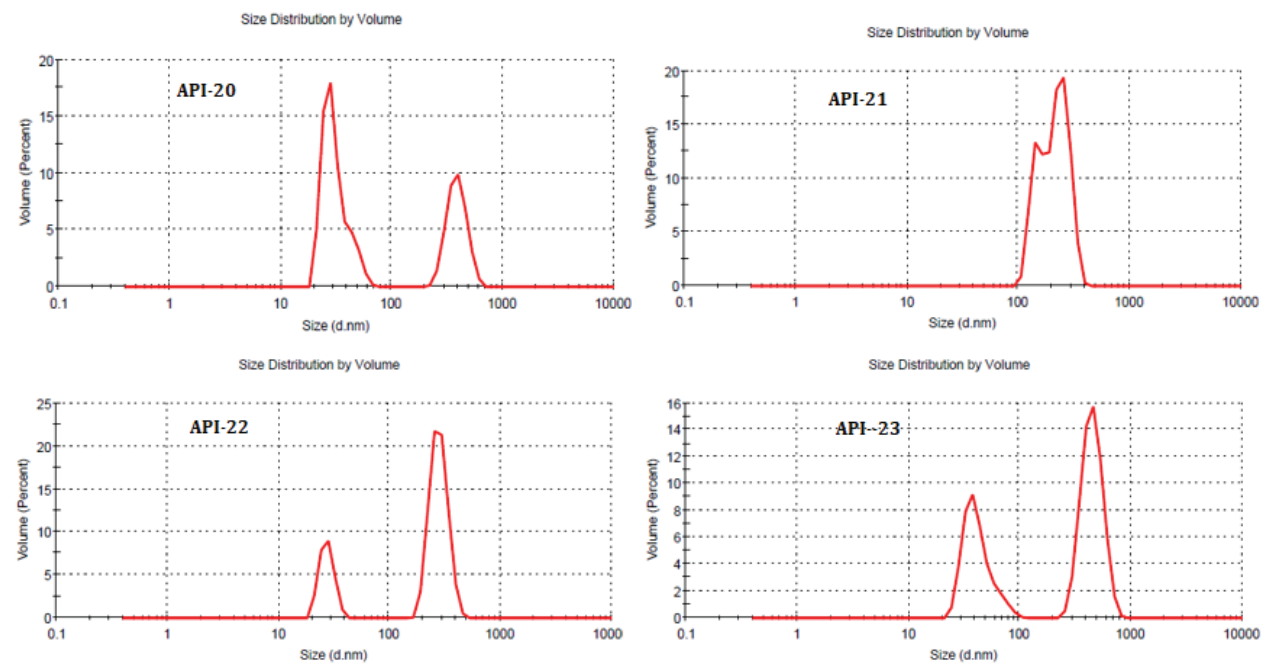
Figure 5. Image displaying results of the four samples about the influence of aqueous silica nanoparticles on (a) emulsions' mean diameter and (b) particle size distribution graphs (volume-based).
