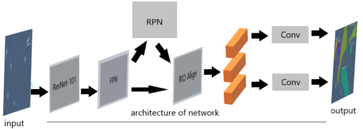
Figure 4.3 General view of Mask R-CNN architecture used on our dataset. Left to right; input image, architecture of network and output image. It takes an input image and returns output image with mask of each instance and their bounding boxes.
