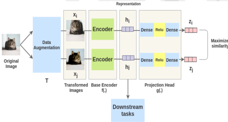
Figure 1.13 Schematic diagram of SimCLR framework [34].
