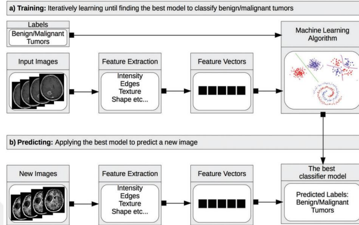
Figure 1.6 Workflow of supervised learning technique [18].
