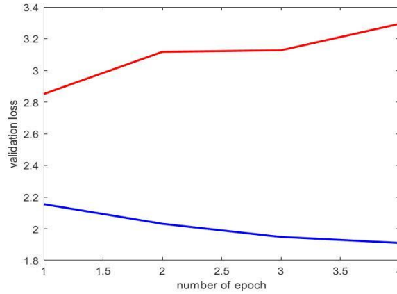
Figure 4.5 Effect of data augmentation on our dataset. Blue color indicates validation loss with augmentation, and red color indicates validation loss without augmentation.
