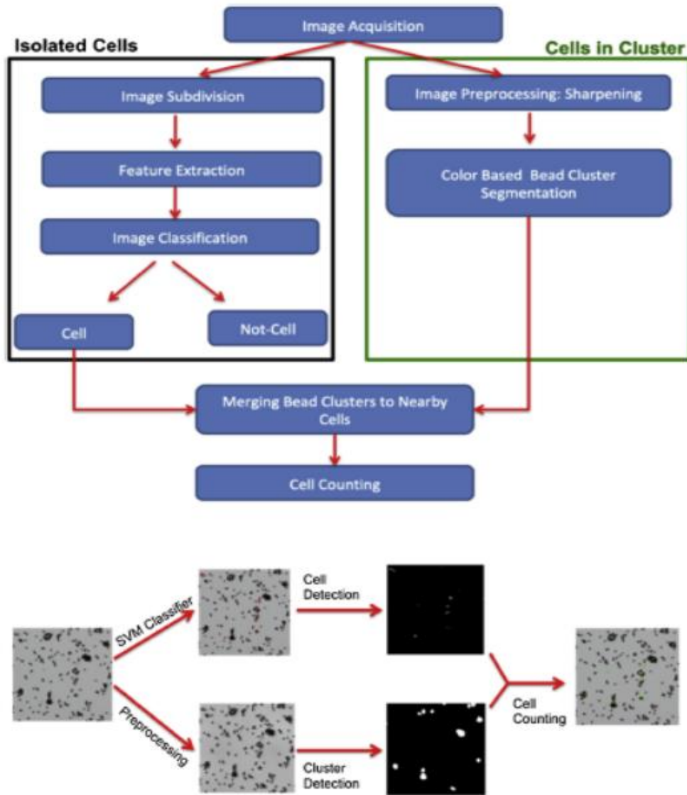
Figure 2.6 Flow diagram of cell detection and counting steps for the images recorded using 20× objective [49].
