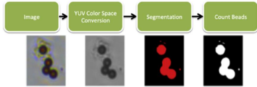
Figure 2.5 The flow diagram of the bead detection using Y channel in YUV color space from the images acquired by the 40× objective [49].
