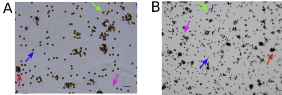
Figure 2.3 Typical optical micrographs of cells and beads recorded using A) 40× objective B) 20× objective. Scale bar indicates 20 \mu m. Blue arrow indicates single beads, pink arrow indicates the cell fragments, green arrow indicates single cell with attached immunomagnetic beads, red arrow indicates fully covered cells with beads as cluster [49].
