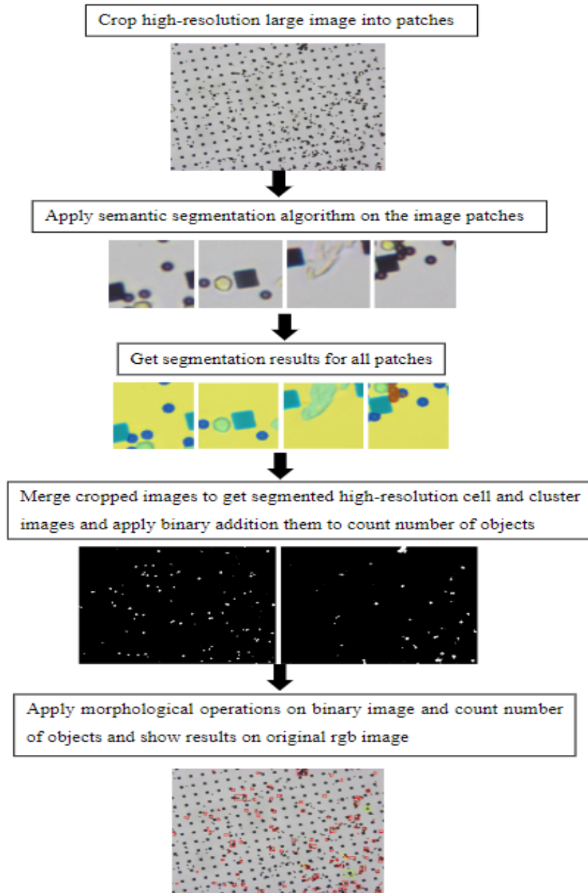
Figure 3.12 Quantification of cells and clusters workflow [99].
