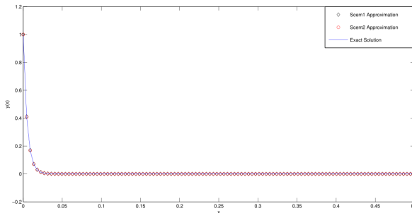
Figure 1. Comparison of the analytical solution and SCEM approximations in solving left symmetric problem for Equations (4.1)–(4.2); \varepsilon = 0.01 . The exact solution and SCEM approximations are almost identical.
