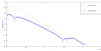
Figure 4. Absolute errors in SCEM approximations y_0^{scem1} and y_1^{scem1} around the boundary layer in solving non-homogeneous problem (4.7)–(4.8); \varepsilon = 0.01 . The second SCEM approximation is superior over the first one.
