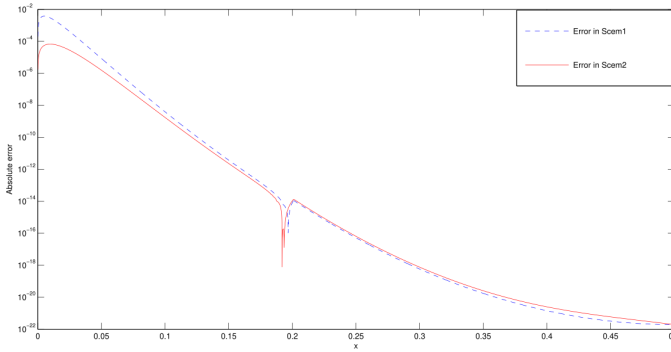
Figure 2. Absolute errors in SCEM approximations y_0^{scem1} and y_1^{scem1} in solving left homogeneous problem (4.1)–(4.2); \varepsilon = 0.01 . The second SCEM approximations is slightly better, as expected.
