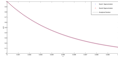
Figure 3. Comparison of the analytical solution and SCEM approximations in solving left symmetric problem for Equations (4.7)–(4.8); \varepsilon = 0.01 . The analytical solution and SCEM approximations are almost identical.
