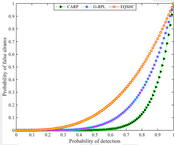
Fig. 2. The probability of false alarms and probability of detection.
