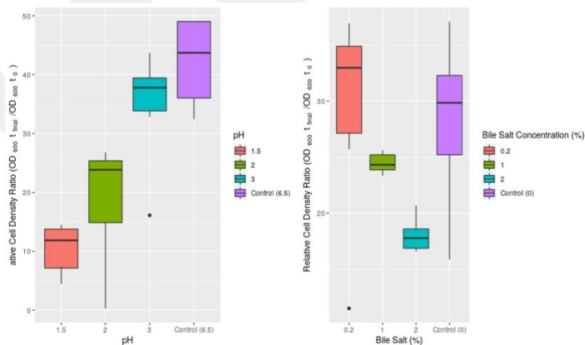
Figure 7. Relative cell density ratios of P. kudriavzevii FOL-04 against various pH and bile salt conditions after 42 hours. OD_{600} values of AGJ at the onset of incubation were as follows: 0.494 \pm 0.02 (control), 0.511 \pm 0.02 (pH 3), 0.470 \pm 0.09 (pH 2), and 0.550 \pm 0.02 (pH 1.5). OD_{600} values of ABJ at the start are following: 0.546 \pm 0.01 (control), 0.593 \pm 0.01 (0.2%), 0.786 \pm 0.02 (1%), and 1.026 \pm 0.06 (2%).
