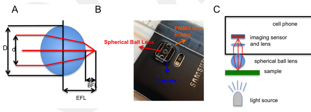
Figure 2. Cell phone microscope using a spherical ball lens. (A) Illustration of the important parameters of the spherical ball lens; (B) Image of the cell phone microscope; (C) Schematic of the measurement.
