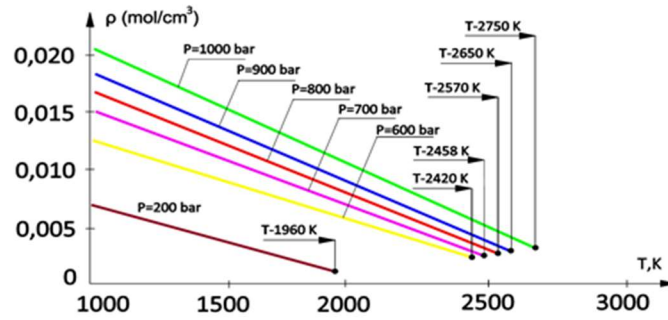
Figure 3. Graph of T- \rho ( P= \text{const.} ) for Hydrogen at the high pressure
