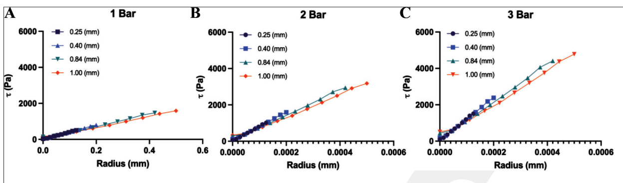
Figure 9. Shear stress profiles as a function of the cylindrical nozzle outlet radius at different inlet pressures. (A) 1 bar, (B) 2 bar, and (C) 3 bar.
