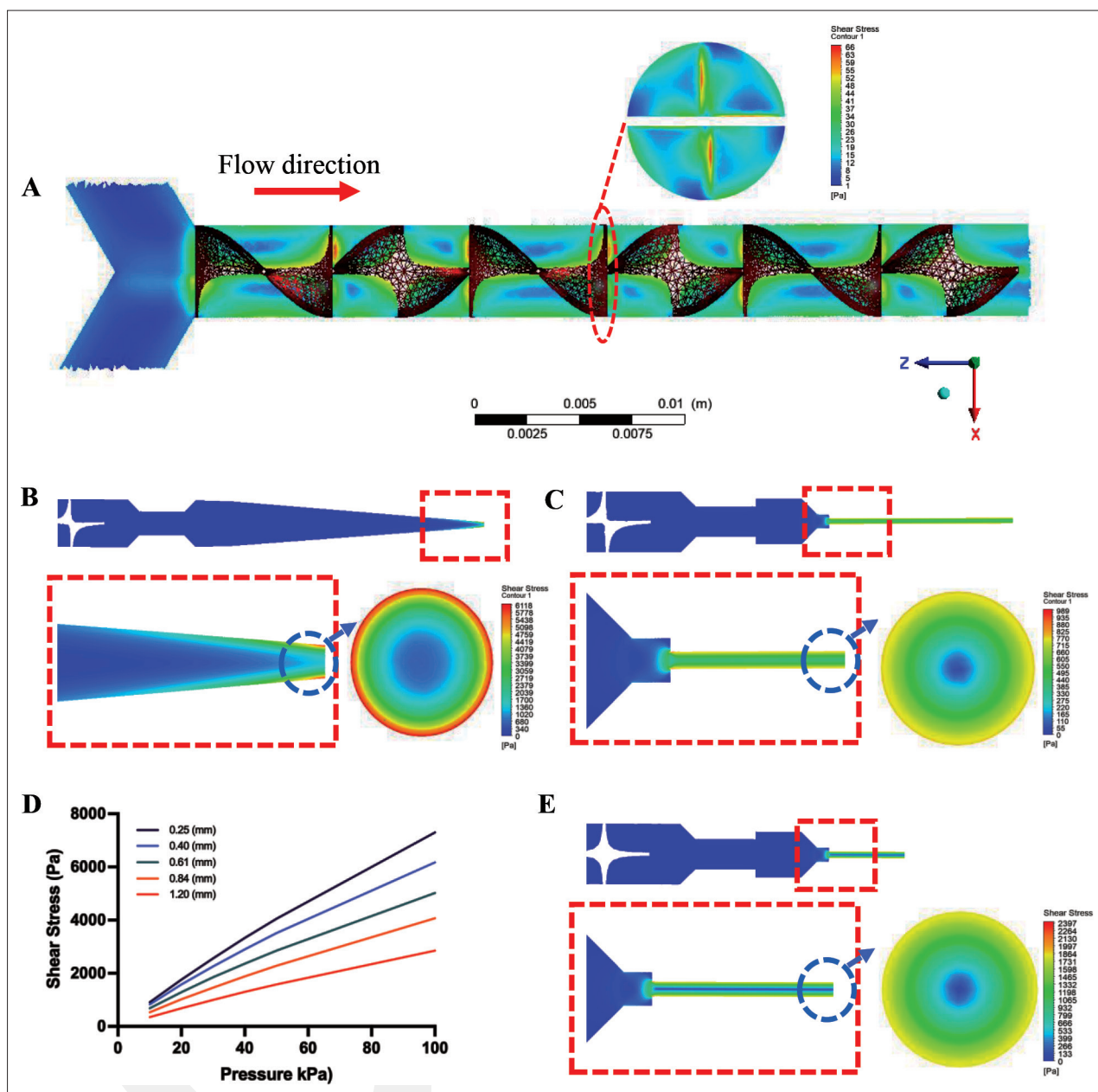
Figure 8. Shear stress distribution results for 1 bar of dispensing pressure. (A) Heat map of the shear stress along the KSM-inserted mixing channel. (B) Conical nozzle with a diameter of 0.4 mm. (C) Long cylindrical nozzle (12mm) with 0.4 mm outlet diameter. (D) Variation of shear stress as a function of applied pressure and nozzle diameter. (E) Contour plot of shear stress for short needle (5 mm).
