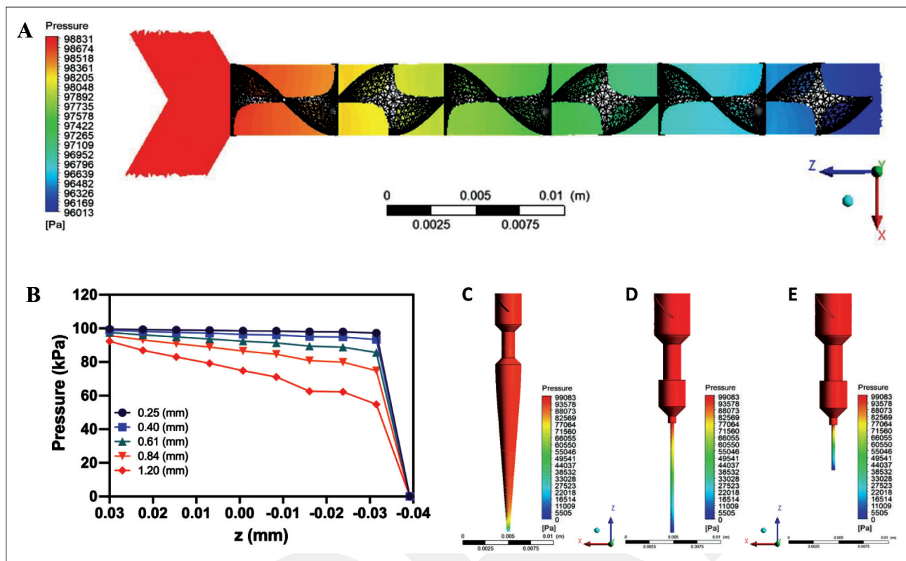
Figure 7. Pressure drop results for an inlet pressure of 1 bar. (A) The local pressure contour plot in the mixing chamber. (B) Variation of pressure along the axial direction of the printing head; contour plots of pressure drop for different nozzle types with outlet diameter of 0.4 mm. (C) Conical needle, (D) long cylindrical needle (12 mm), and (E) short cylindrical needle (5 mm).
