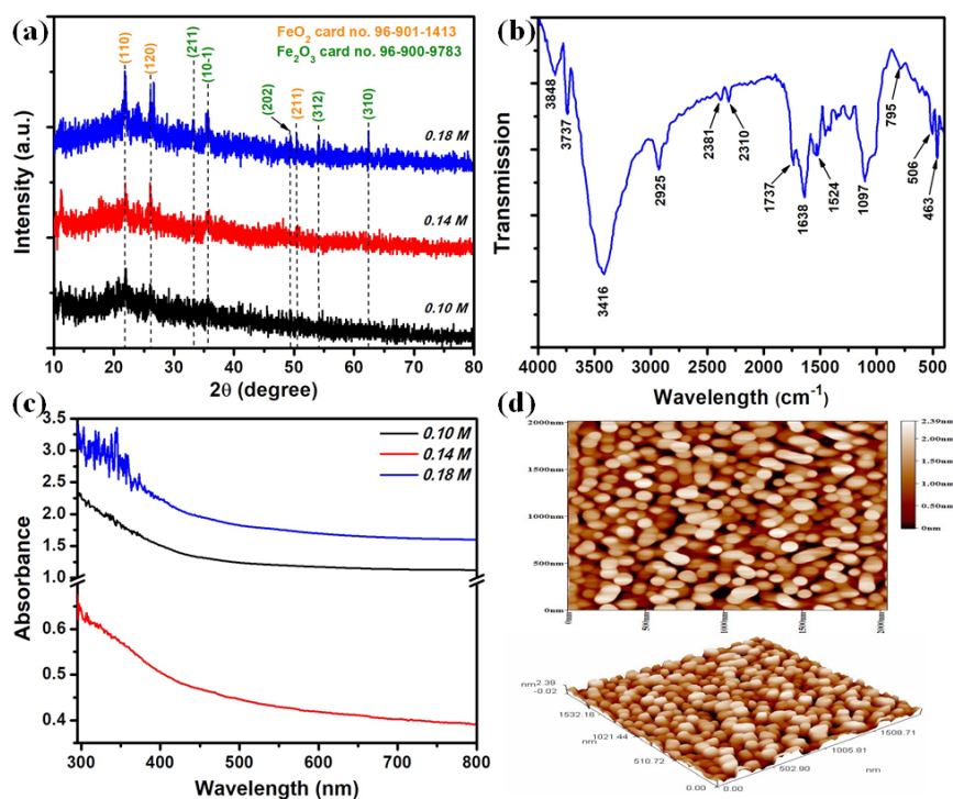
Figure (2): (a) XRD patterns, (b) FT-IR spectra, (c) UV-vis spectra, and (d) AFM of 2D and 3D images of the prepared NPs.
