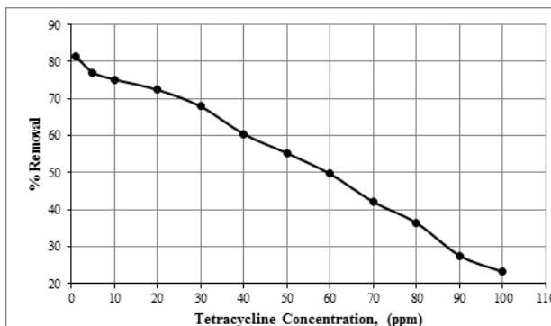
Figure 2 Effect of initial concentration on the percentage removal of tetracycline antibiotic
