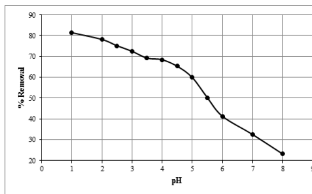
Figure 3 Effect of pH on the percentage removal of tetracycline antibiotic
