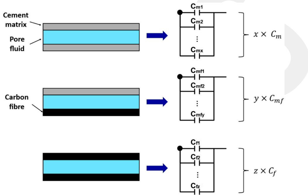
Fig. 14. Solid-liquid phases to construct layered capacitor in a cement-based sensor: C_m is the cement-pore fluid-cement layered capacitor, C_{mf} is the cement-pore fluid-fibre layered capacitor, C_f is the fibre-pore fluid-fibre layered capacitor, x , y , and z are their numbers, respectively.
