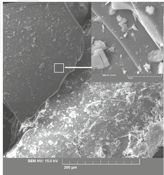
Fig. 3 SEM image of pure Vermiculite
