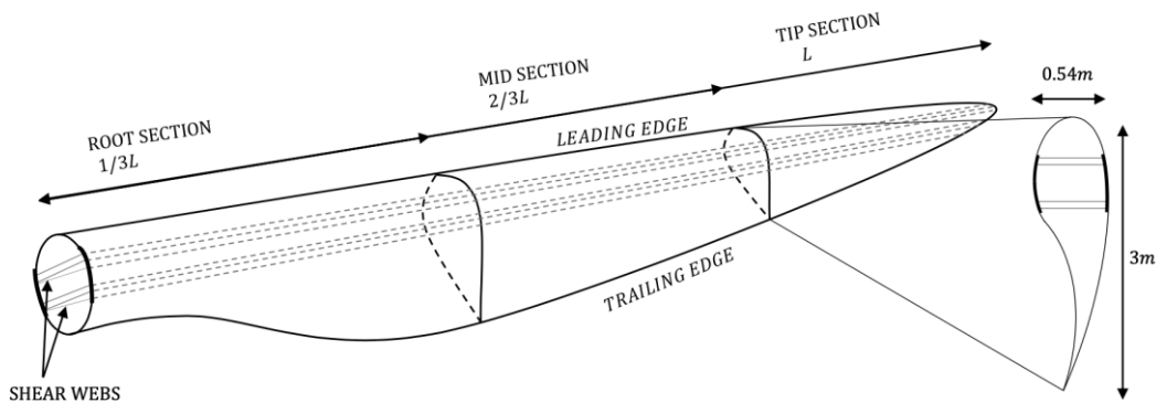
Figure 2. Dimensions of a sample 61.5 m Wind Turbine Blade from Ref. [9].
