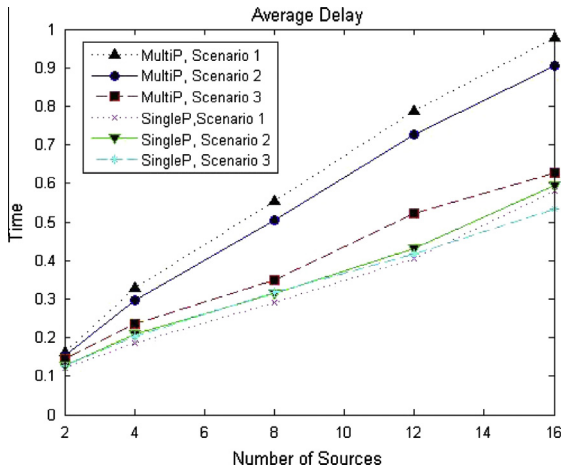
Fig. 5. Average delays of single-path and multi-path routing.
