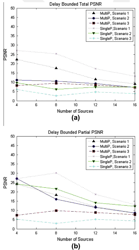
Fig. 3. (a) The delay bounded average PSNR values of the whole image, (b) the delay bounded average PSNR values of the partial image for four different flow numbers. Deadline is set to 2.0.
