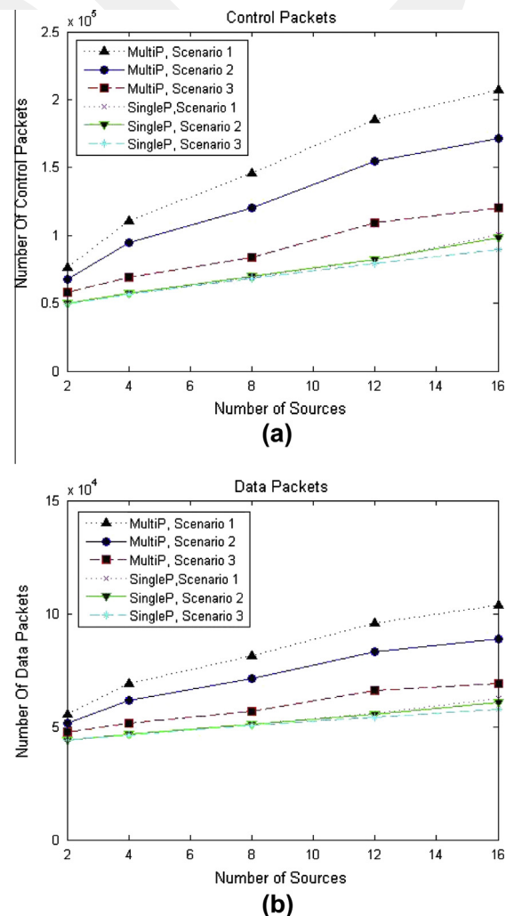
Fig. 4. (a) Number of control packets, (b) number of data packets for 5 different flow numbers.
