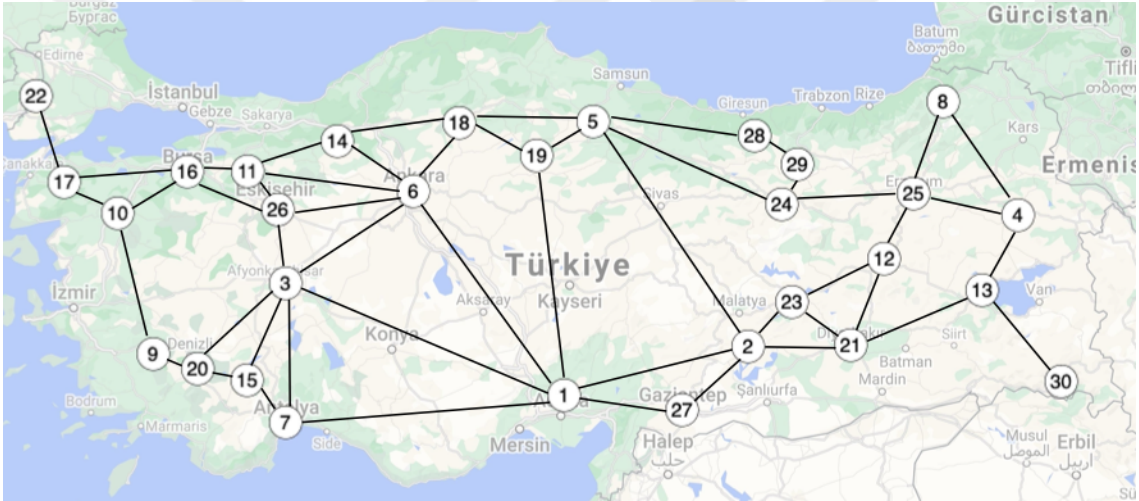
Figure 2.1. Non-complete transportation network consisting of 30 cities of Turkey.
