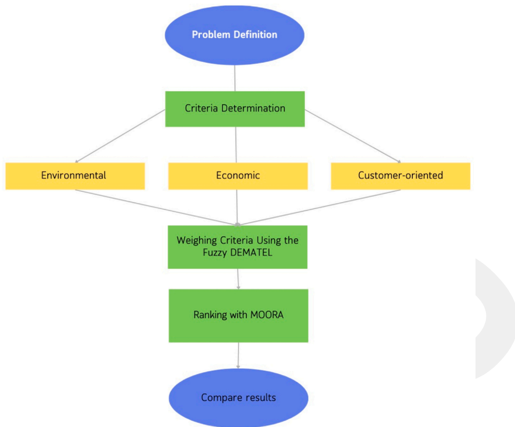
Fig. 1. Research Methodology.
