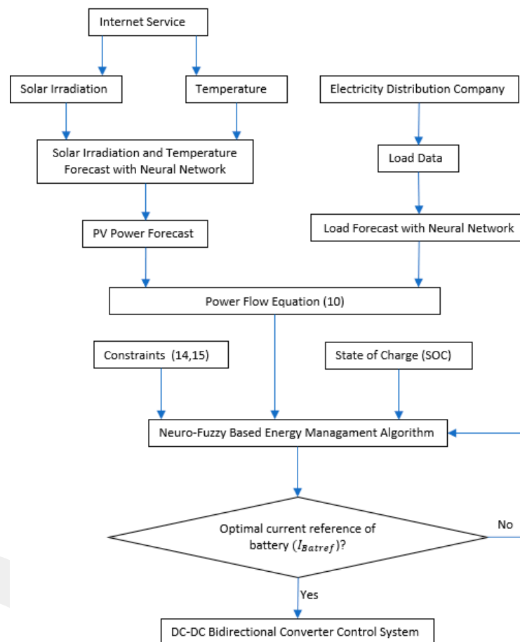
Figure 9. MPC-inspired energy management algorithm flowchart.
