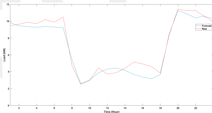
Figure 13. Forecasting and real load curves for 04/02/2019.
