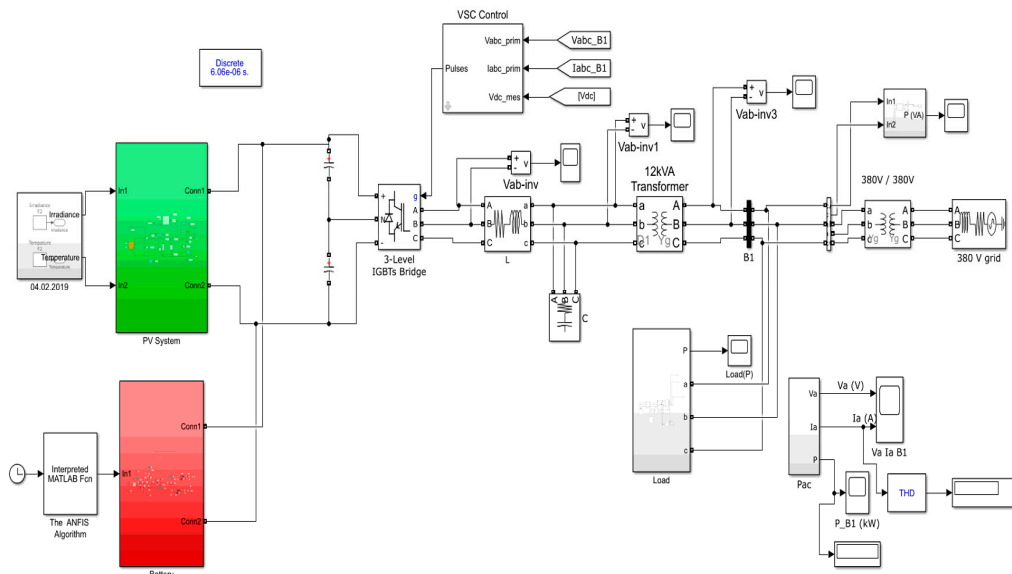
Figure 3. Matlab/Simulink block diagram of the designed microgrid system.
