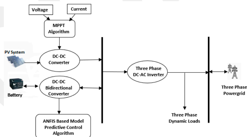
Figure 1. Structure of the designed microgrid system.
