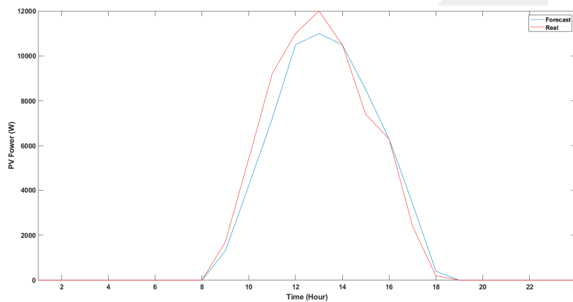
Figure 12. Forecasting and real PV power curves for 04/02/2019.
