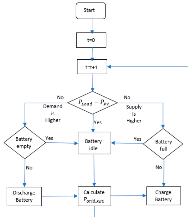
Figure 7. Rule-based control flowchart [56].
