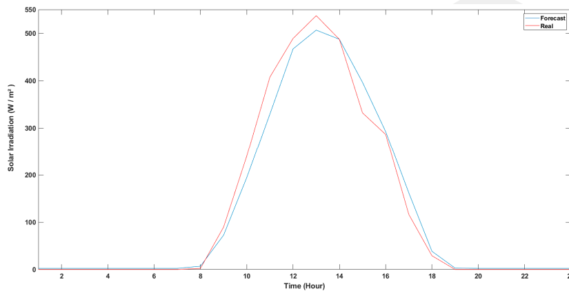
Figure 10. Forecasting and real solar irradiation curves for 04/02/2019.
