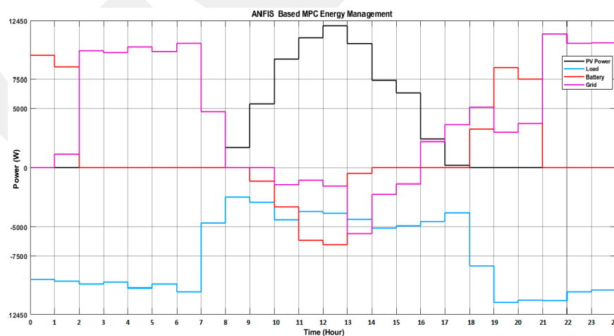
Figure 15. Power dispatching using with ANFIS-based MPC-inspired energy management for 04/02/2019.
