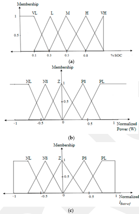
Figure 8. The fuzzy sets of (a) SoC (state of charge), (b) power and (c) battery current.
