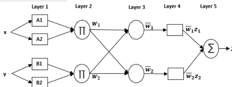
Figure 6. Typical architecture of adaptive neural fuzzy inference system (ANFIS) [54,55].
