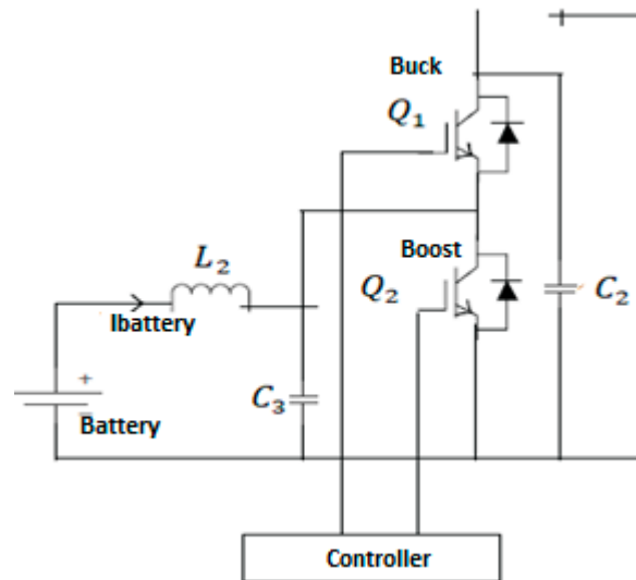
Figure 2. Structure of the DC–DC bidirectional converter.
