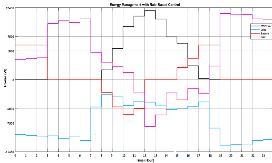
Figure 14. Power dispatching using energy management with rule-based controller (RBC) for 04/02/2019.
