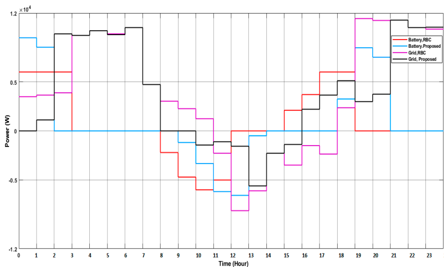
Figure 16. Comparison of battery usage and grid usage.
