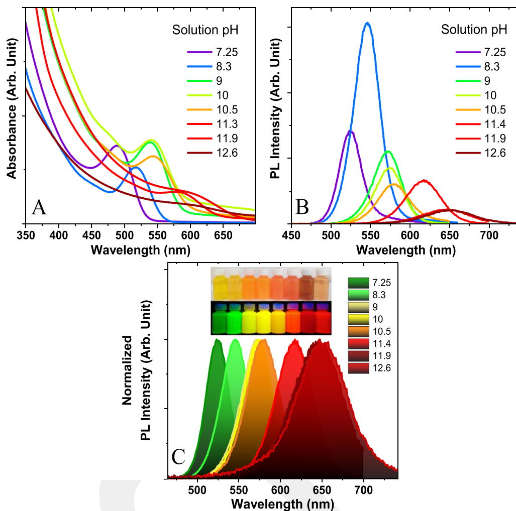
Figure 5. (A–C) UV–Vis absorption, PL emission, and normalized PL emission ( \lambda_{\text{exc}} = 380 \text{ nm} ) spectra of colloidal ZnCdTeS NCs prepared at different pH values, while other experimental parameters such as the molar ratio of precursors (Cd:Zn:NAC:TSC:Te = 1:1.5:0.7:0.9:0.36), refluxing temperature ( 100^\circ\text{C} ), and reaction time (2 h) were constant. Inset shows the digital images of ZnCdTeS NCs under daylight (up) and 365 nm/12 W UV irradiation (down).
