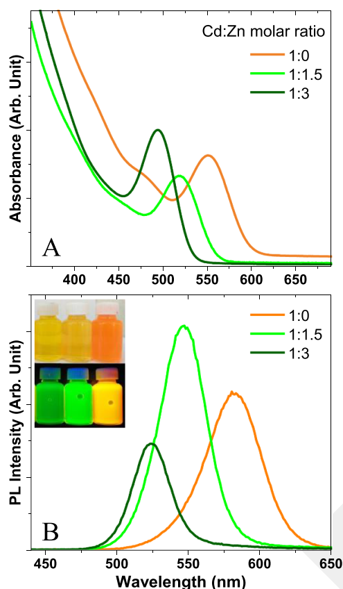
Figure 6. (A, B) UV-Vis absorption and PL emission ( \lambda_{exc} = 380 nm) spectra of colloidal ZnCdTeS NCs prepared at different Cd:Zn molar ratios, while other experimental parameters were constant. Insets show the digital images of ZnCdTeS NCs under daylight (up) and 365 nm/12 W UV irradiation (down).
