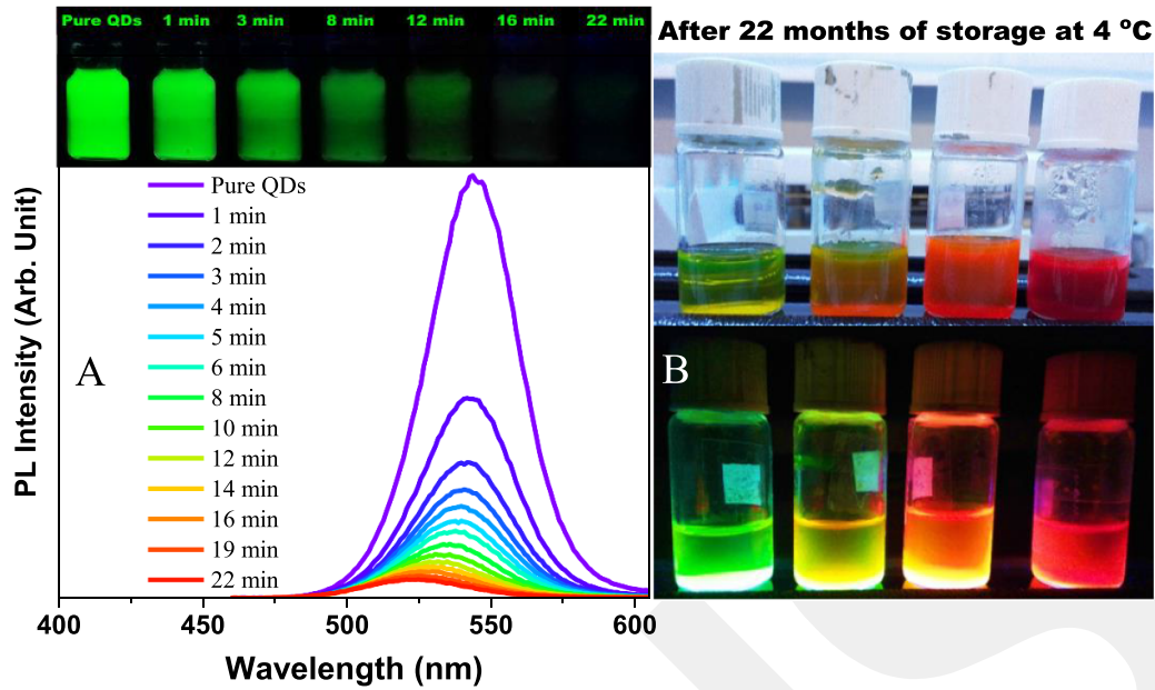
Figure 7. (A) Temporal evolution of the PL emission ( \lambda_{exc} = 380 nm) spectrum of optimized ZnCdTeS NCs after addition of H_2O_2 solution. Inset shows the digital images of ZnCdTeS NCs under 365 nm/12 W UV irradiation after addition of H_2O_2 . (B) Digital images of samples prepared at different reaction times, after 22 months storage at refrigerator (under daily light and UV irradiation).
