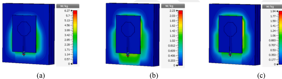
Fig. 16. SAR values of the designed antenna without the MM structure at its back calculated in simulations for 10 g human body tissue at a frequency of (a) 4 GHz, (b) 7.5 GHz, and (c) 10.5 GHz.
