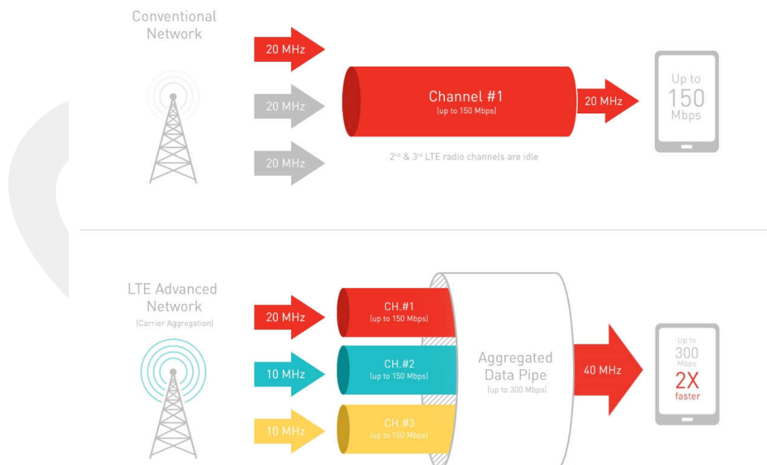
Figure 2.2 Carrier Aggregation [27]
