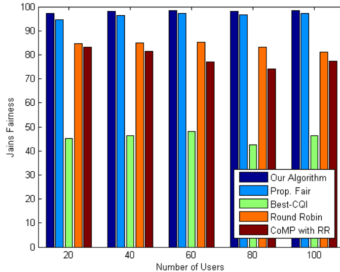
Figure 6.5 Jain's Fairness Index of the Schedulers
