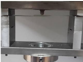
(c) normal impact test condition
