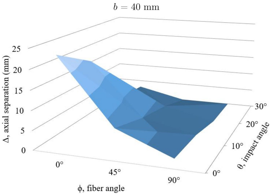
Fig. 11 Effects of fiber angle and impact angle on axial separation of composite single-lap joints ( b : overlap length)
