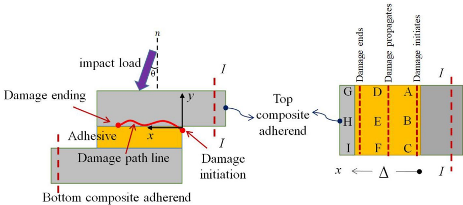
Fig. 12 Schematic representation of microscope images of the fracture surfaces of joints (Figs. 13, 14, and 15)
