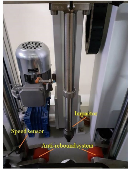
(b) impact device components
