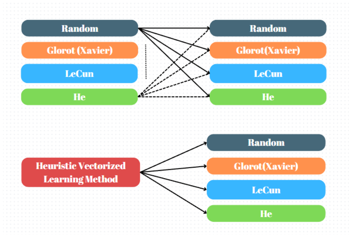
Figure 3.2 Weight Assignment Scheme on Generated Algorithm
