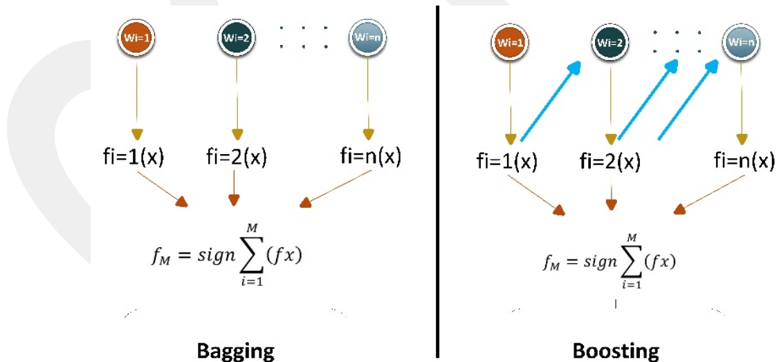
Figure 2.2 Bagging and boosting methods
