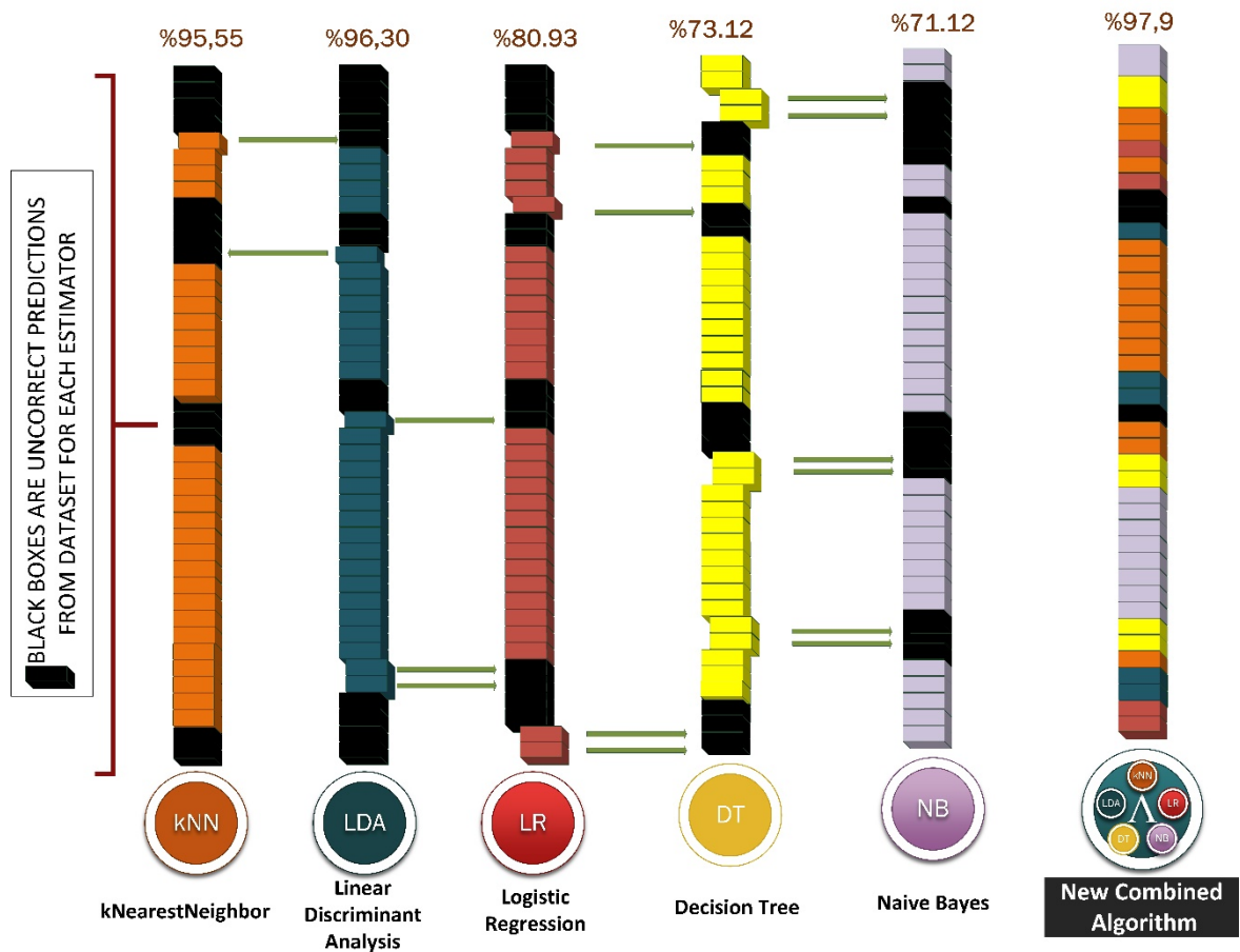
Figure 2.4 PSO effects for each ML algorithm
