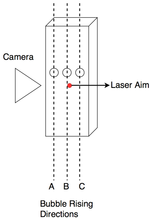
Figure 4.3.3 Bubble motion inside of glass cuvette. If a bubble passed through A direction, its radius appeared larger in images. If a bubble passed through B or C its radius appeared smaller than A direction.
