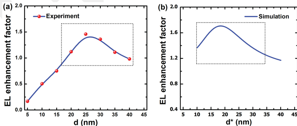
Figure 5. a) Experiment and b) simulation results. Electroluminescence enhancement factor for the QDs in the presence of Ag nanoislands. d and d^* present the surface-to-surface and center-to-center distance between the QDs and MNPs, respectively.
