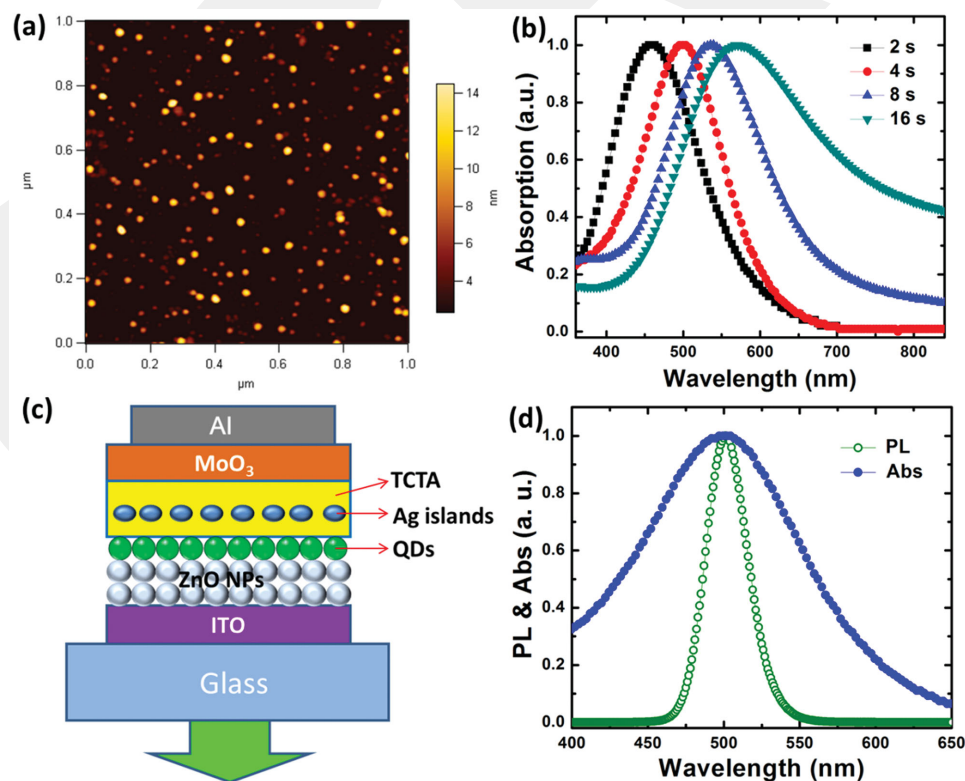
Figure 1. a) AFM image of Ag nanoislands formed on ITO substrate. b) Absorption spectra of Ag nanoislands with different deposition time. The Ag nanoislands were deposited with a fast deposition rate of 0.375 \text{ nm s}^{-1} . c) Schematic of the device configuration of the QLEDs embedded Ag nanoislands. d) Absorption spectrum of the Ag nanoislands and PL spectrum of the green QDs excited at 400 nm.
