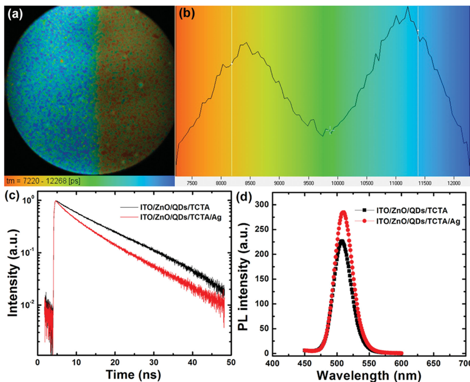
Figure 3. a) FLIM image of CdSe/ZnS QDs films recorded upon excitation at 400 nm. The QDs layer without Ag nanoislands is shown in the bright color while QDs covered by Ag nanoislands is shown in the dark color. b) Statistical lifetime distribution (ns) within the whole area of measurement. The lifetime of QDs covered by Ag nanoislands is shortened. c) Time-resolved fluorescence spectra of QD films with and without nanoislands. d) PL intensity of QD films with and without Ag nanoislands excited under 400 nm.
