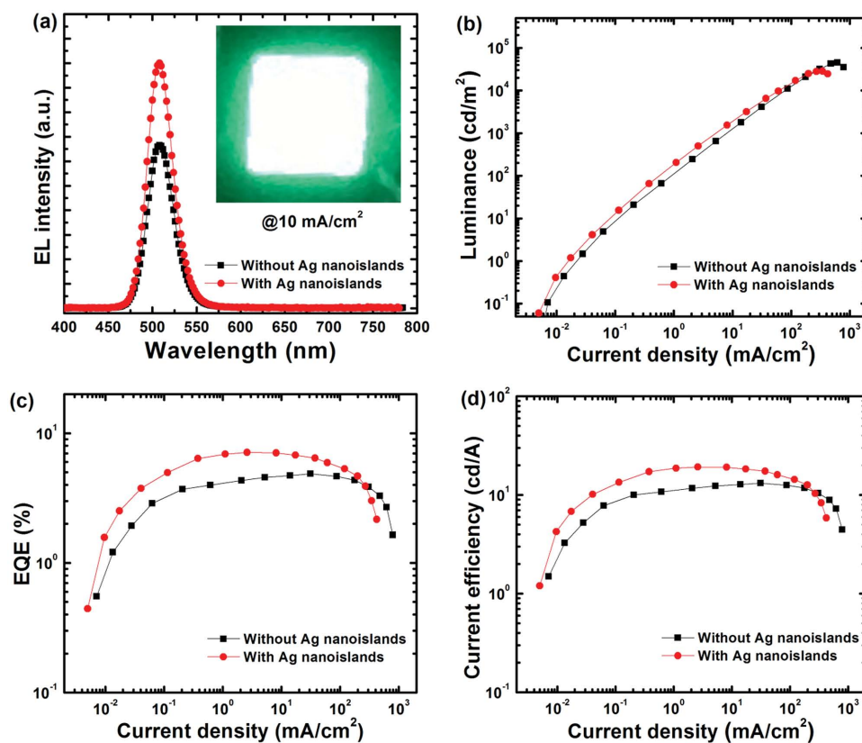
Figure 2. a) EL spectra of a typical plasmonic QLED with Ag nanoislands and the reference device without Ag nanoislands. Inset: The photographic image of the plasmonic QLED. Comparison of b) luminance, c) EQE, and d) CE for the plasmonic and reference devices as a function of the current density.
