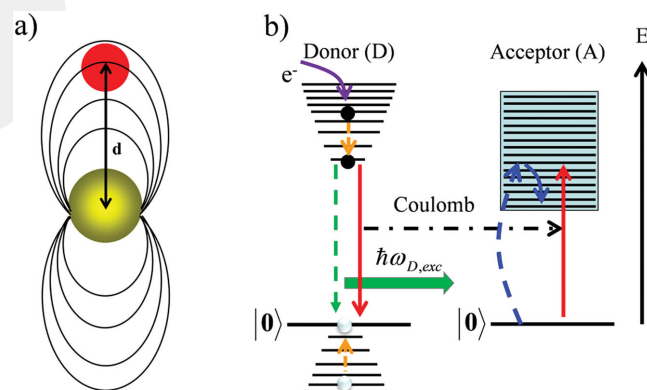
Figure 4. a) Surface plasmon enhanced QD emission. b) Energy diagram for the donor–acceptor (D–A) pair energy transfer process. Purple solid line represents the electron and hole injection. Orange dashed line represents the electron and hole relaxation process. Green dashed lines show light emission process (relaxation from the lowest excited state to the ground state). Red solid lines represent the energy transfer from the donor to the acceptor. Horizontal dashed black line shows the Coulomb interaction between the donor and acceptor. Blue dashed lines represent the absorption process of the acceptor.
