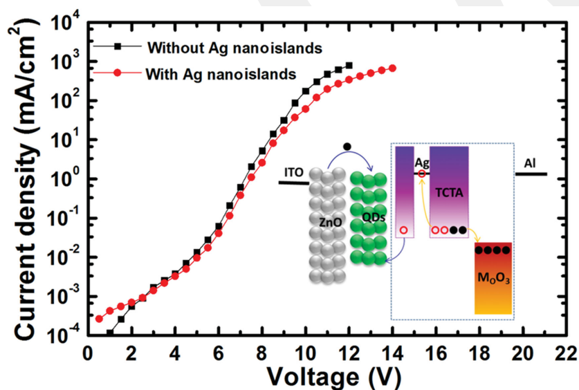
Figure 6. Electric characteristics of QLEDs with and without Ag nanoislands. Inset: Energy level diagram of the QLEDs embedded Ag nanoislands. Red hollow circles represent holes. The hole injection from anode to the TCTA results from carrier breakthrough from the \text{MoO}_3 /TCTA junction. Black solid circles represent electrons. The electrons are injected from the Al to the QD layer via the conduction band of the ZnO nanoparticle layer.
