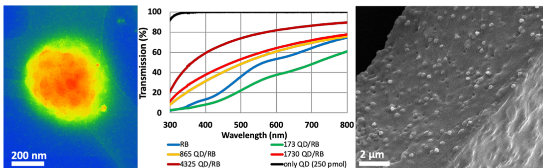
Figure 6. (Left) Colored HAADF STEM image of RB and quantum dot (QD) hybrid (4325 quantum dots per RB particle sample). (Middle) Transmission spectra of the films made of quantum dot and RB particles hybridized at different number ratios. (Right) SEM image of the RB particle and quantum dot hybrid (4325 quantum dots per RB particle sample).
